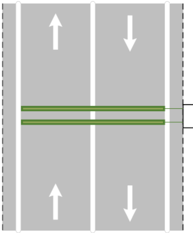
Figure 7.3.3.1 – Typical Piezo-Piezo configuration for bicycle counter
