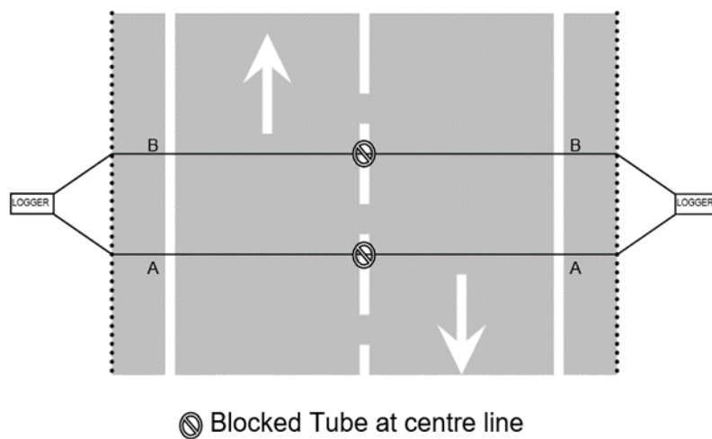
Figure 7.3.1.1(a) – Preferred method for surveying single carriageway bi-directional site
