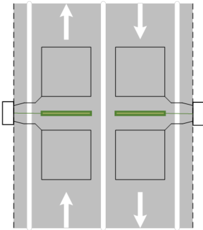
Figure 7.3.2.2.2 – Typical loop-piezo-loop configuration on single carriageway bi-directional road
