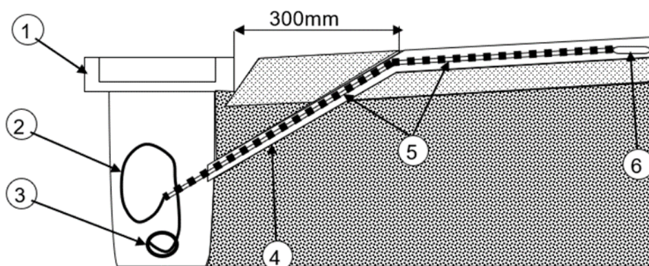
Figure 7.4.2.2(c) – Piezoelectric installation details (feeder cable to pit arrangement)
