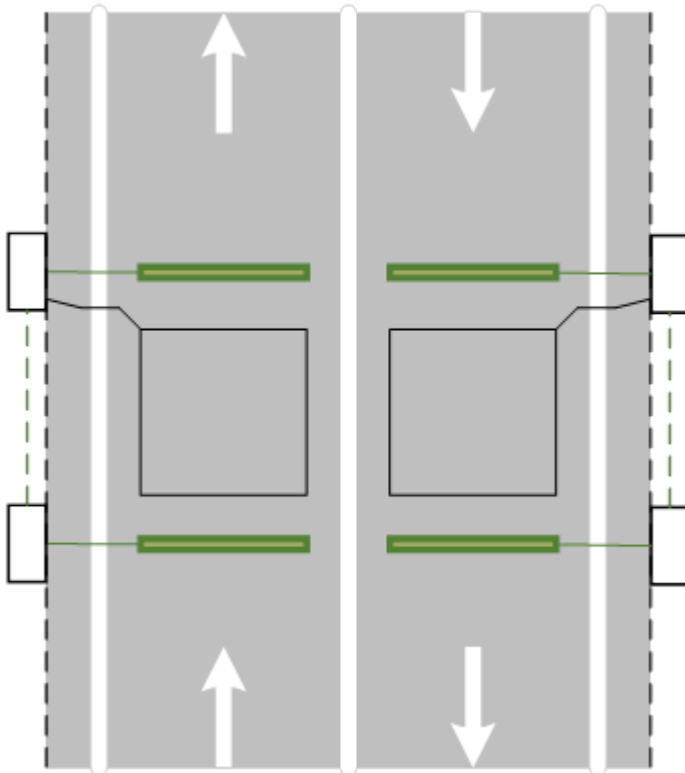
Figure 7.3.2.1(a) – Typical Piezo-Loop-Piezo configuration on single carriageway bi-directional road
