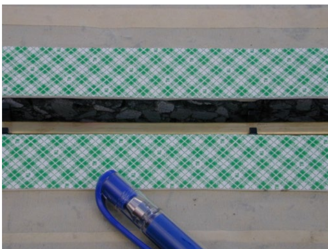
Figure 7.4.4(e) – Piezoelectric installation details (preparation of sealant feeder slot continuation)
