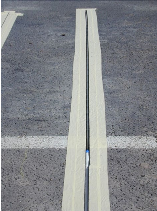
Figure 7.4.4(d) – Piezoelectric installation details (preparation of sealant feeder slot)
