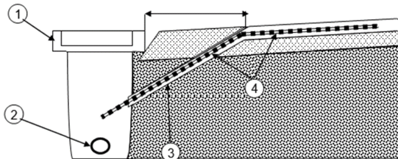
Figure 7.4.4.2(b) – Piezoelectric installation details (feeder slot to pit arrangement)
