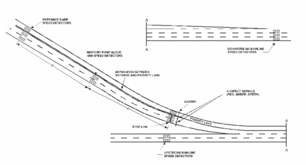
Figure 6.1.2.2(d) – Complex entry-ramp, 2 lanes of metered traffic and a metered priority lane
