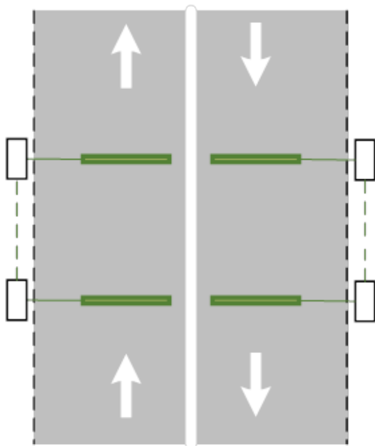
Figure 8.3.3 – Single lane bi-directional carriageway (Piezo-Piezo configuration for weigh-in-motion sites)
