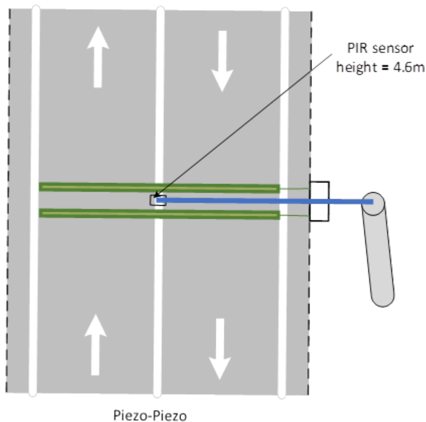
Figure 7.3.3.2 – Typical configuration for combined bicycle / pedestrian counter
