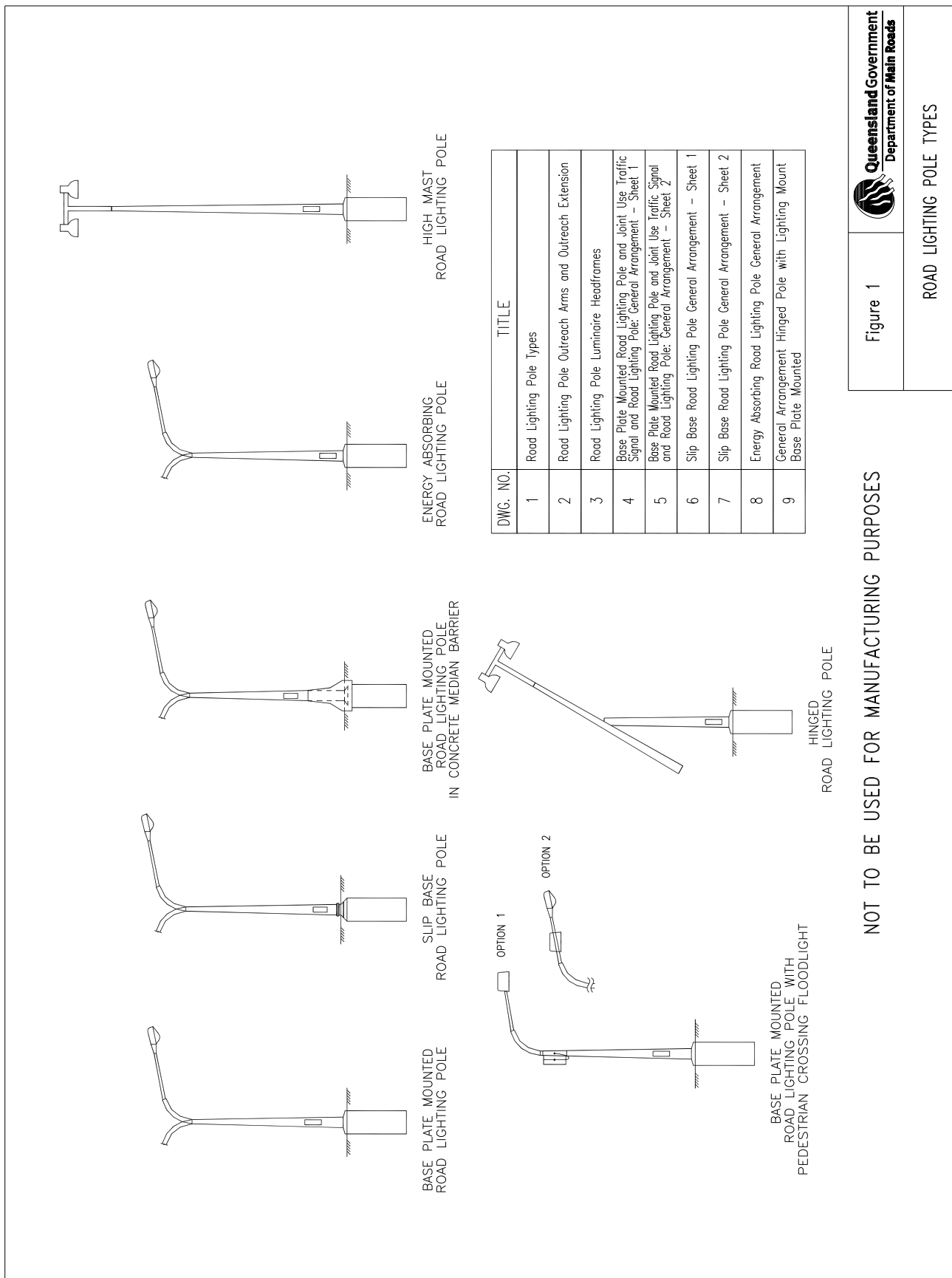
Figure 1 – Road Lighting Pole Types
