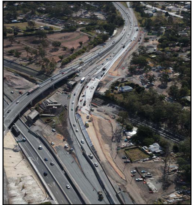
Construction of the new Warrego Highway eastbound bridge
