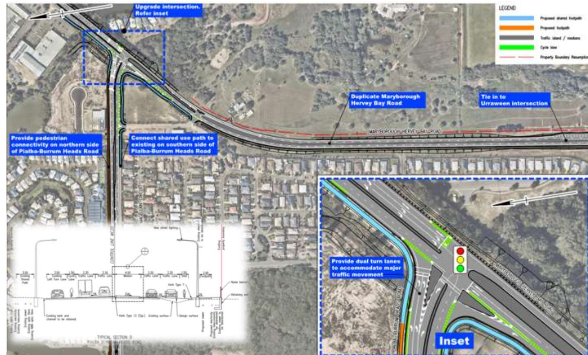
Image: Aerial and Drawing: Maryborough – Hervey Bay Road and Pialba – Burrum Heads Road intersection. Source: Maryborough – Hervey Bay Road and Pialba – Burrum Heads Road business case, TMR.
