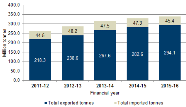
Queensland Total Throughput 2011-12 to 2015-16
