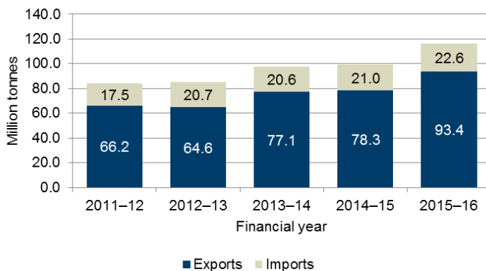
Gladstone Total Throughput
