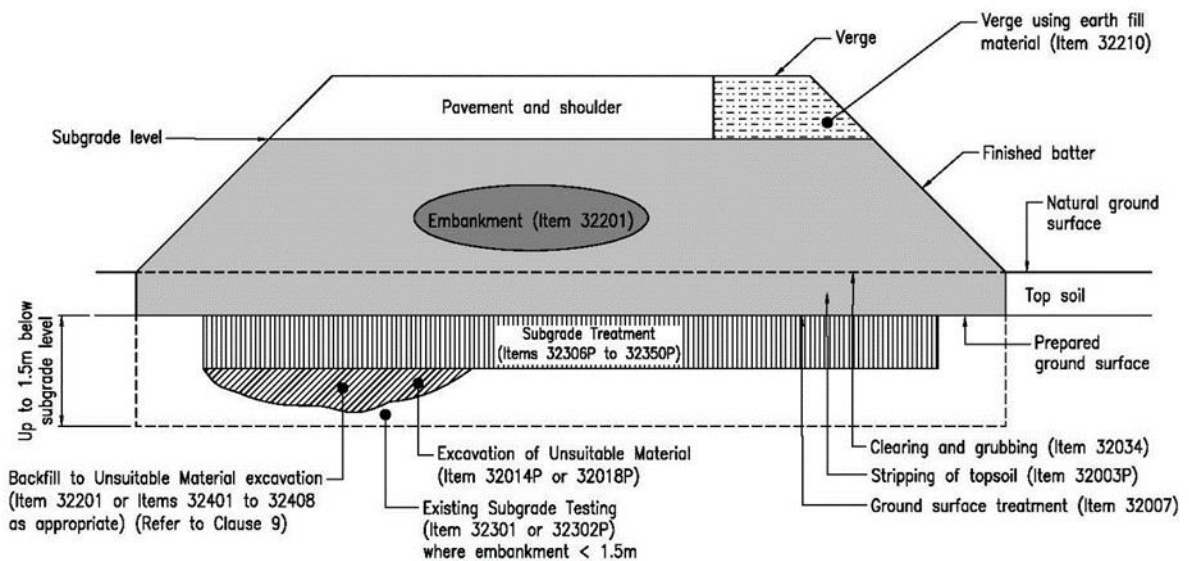
Figure 2.1(b) – Embankment
