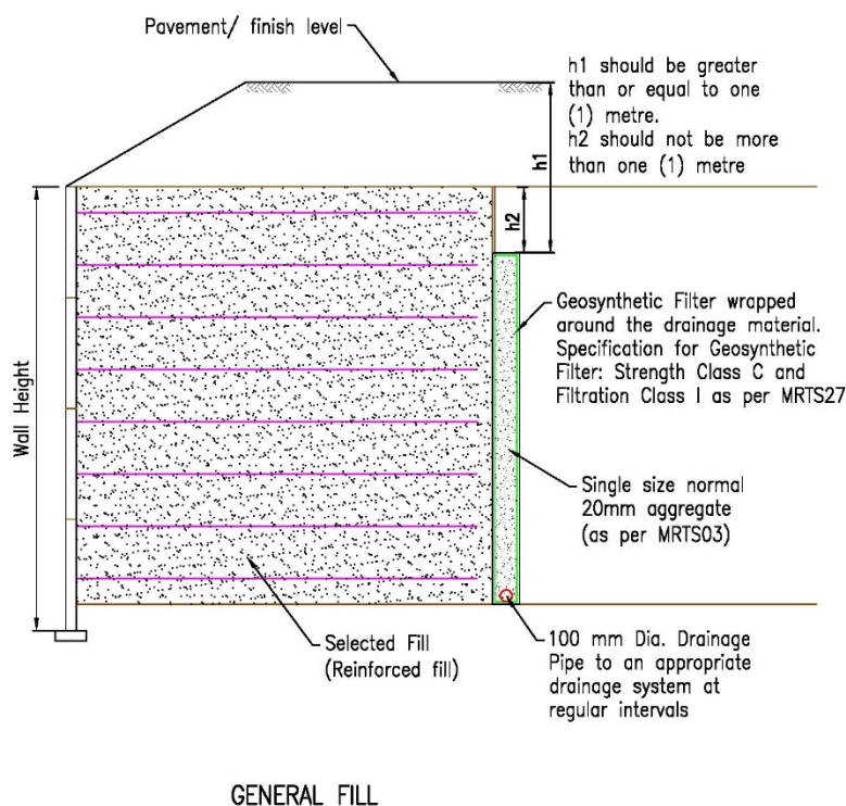
Figure 8.2 – Typical details of a drainage blanket behind RSS block
