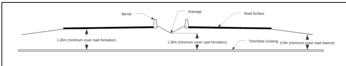
Figure 6.2.5(b) - Minimum depth below dual carriageway
