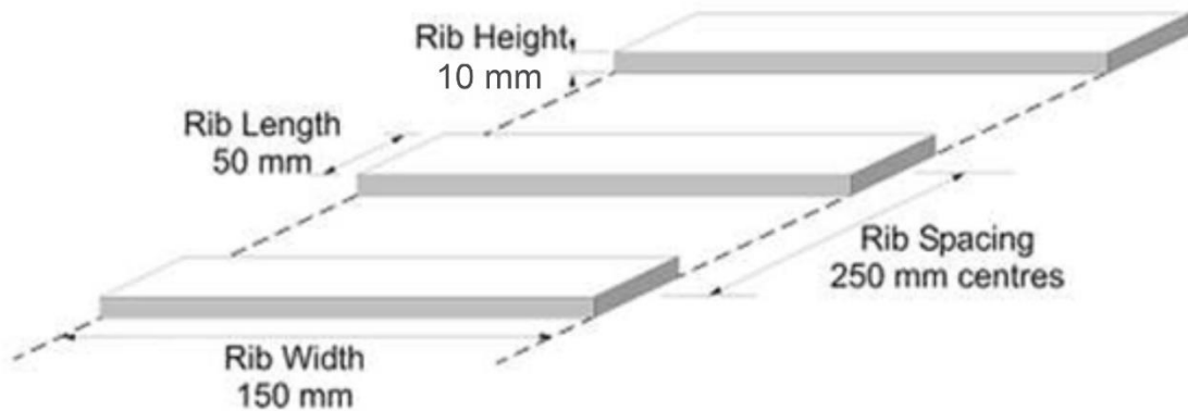
Figure 7.7.3(a) – ATLM edge line
