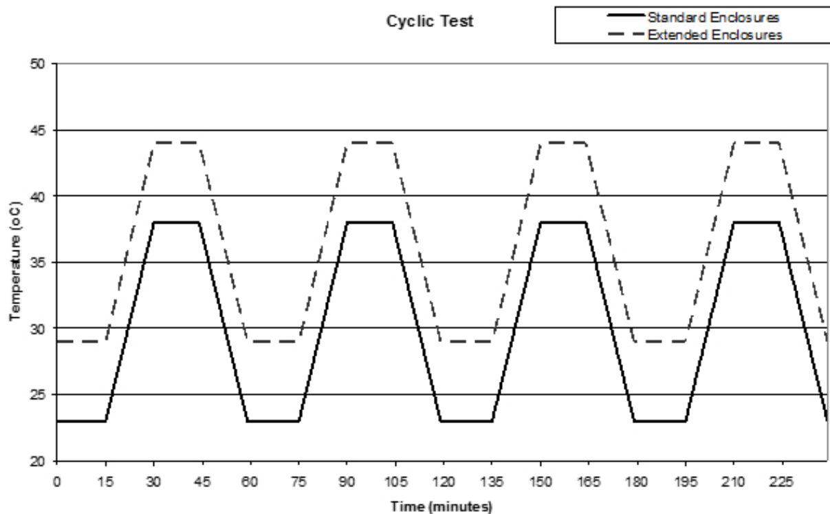
Figure B8.3.2 – Cyclic Test Procedure
