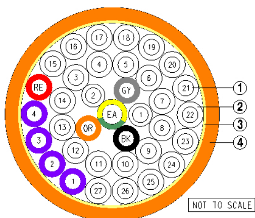
Figure 6.5 – 36-core cable
