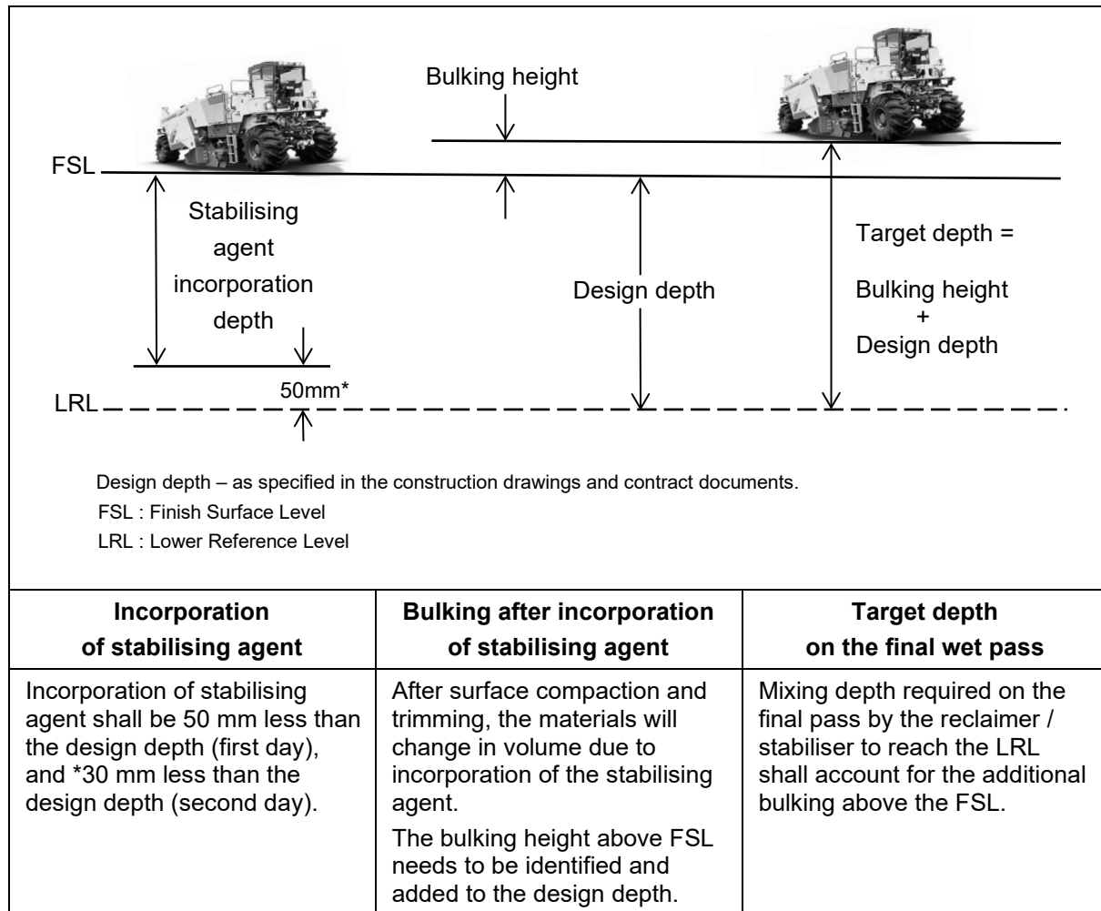
Figure 8.6.6.4 – Target depth sketch
