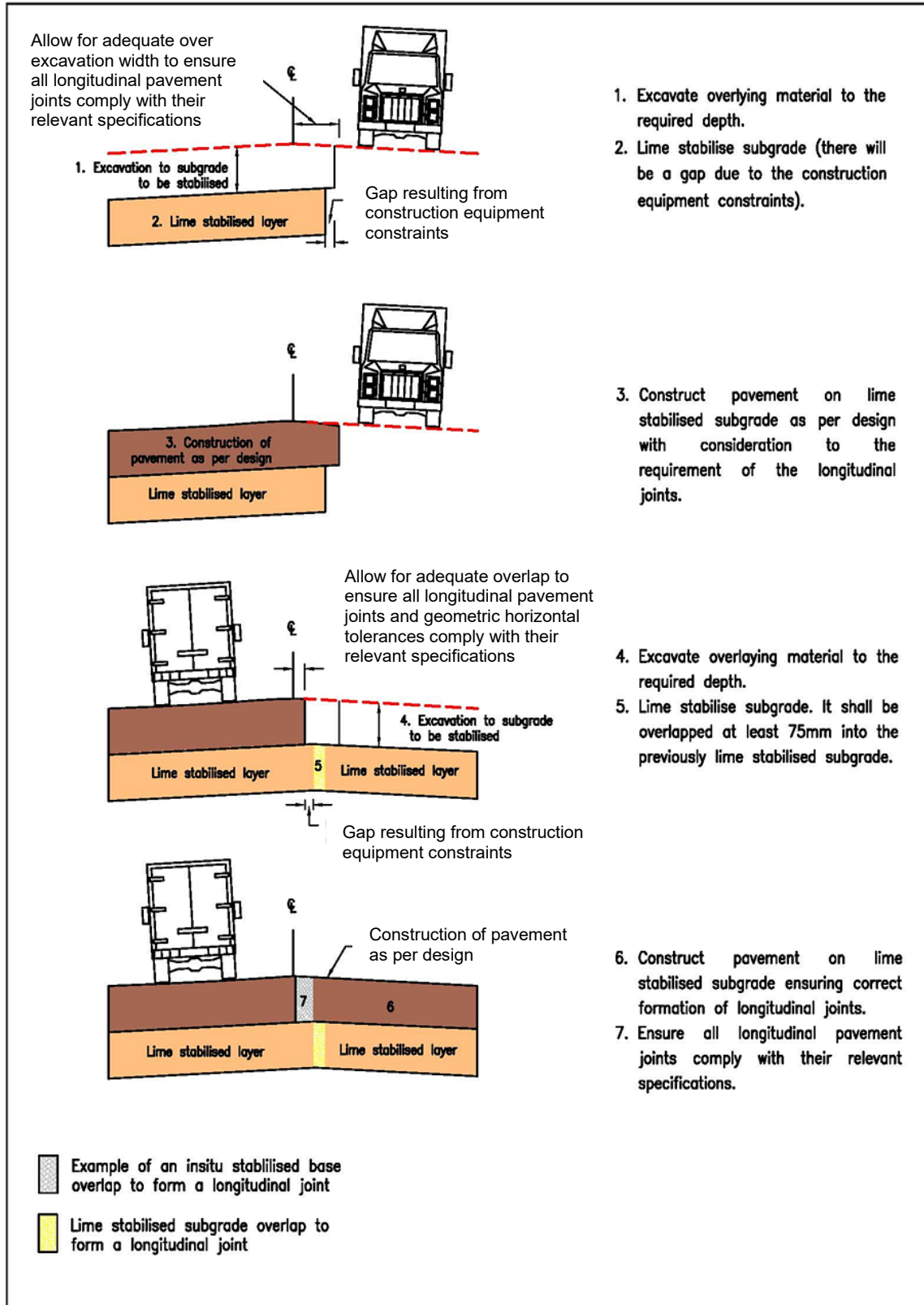
Figure 8.6.7.2 – Typical construction process
