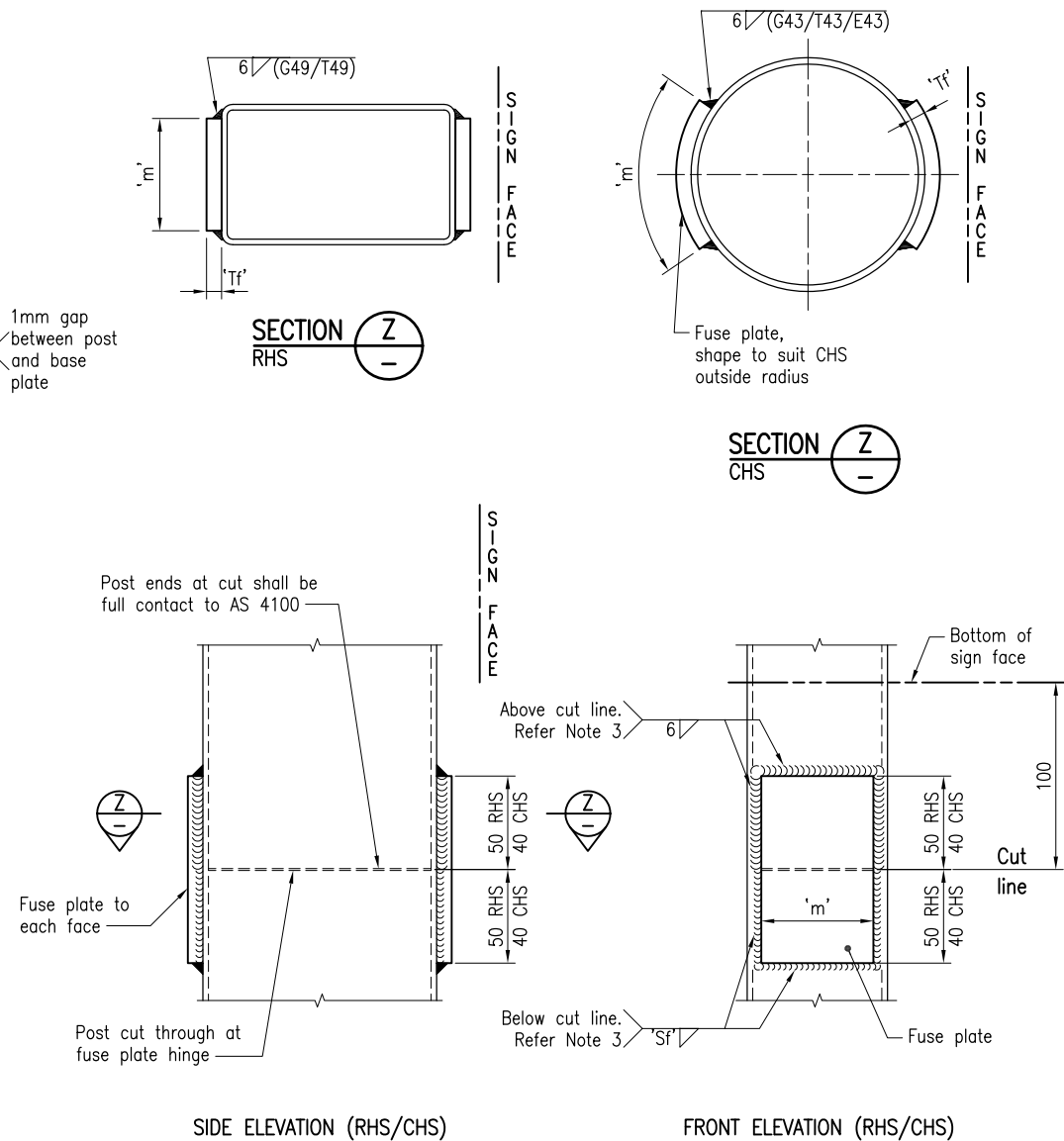
DETAIL E FUSE PLATES DETAIL (TWO OR MORE SUPPORTS ONLY)
