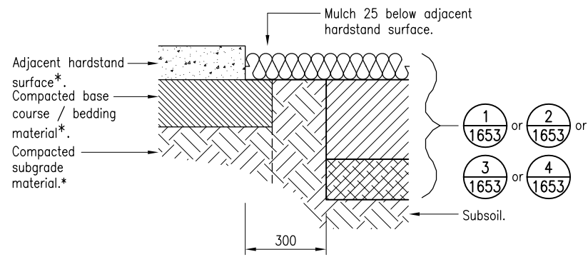
DETAIL 1 1644 HARDSTAND ABUTMENT TO PLANTING BED
