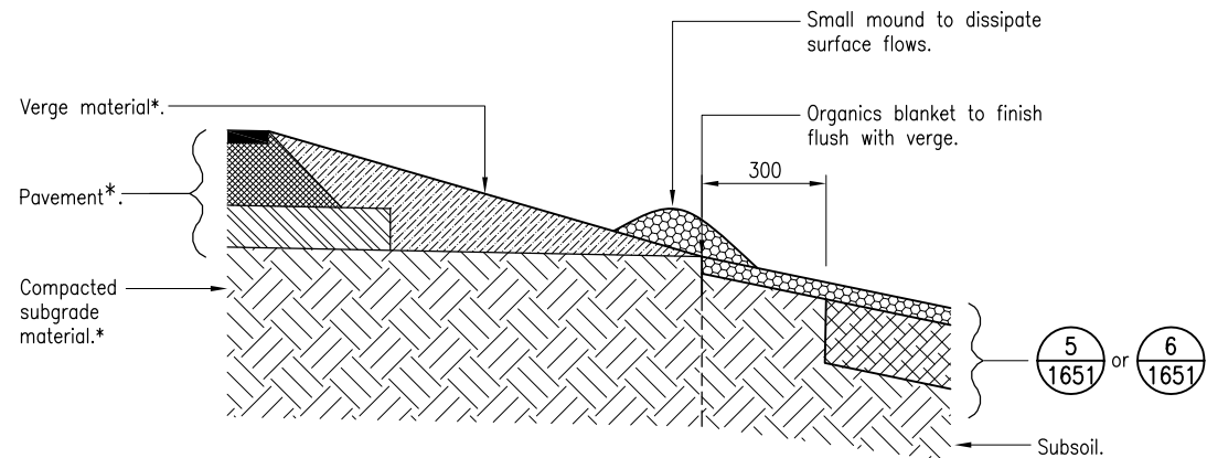
DETAIL 7 1644 VERGE TO ORGANICS BLANKET
