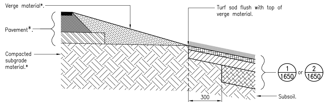
DETAIL 5 1644 VERGE TO TURF
