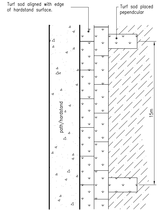
DETAIL 8 1644 PLAN - HARDSTAND ABUTMENT TO SEEDING
