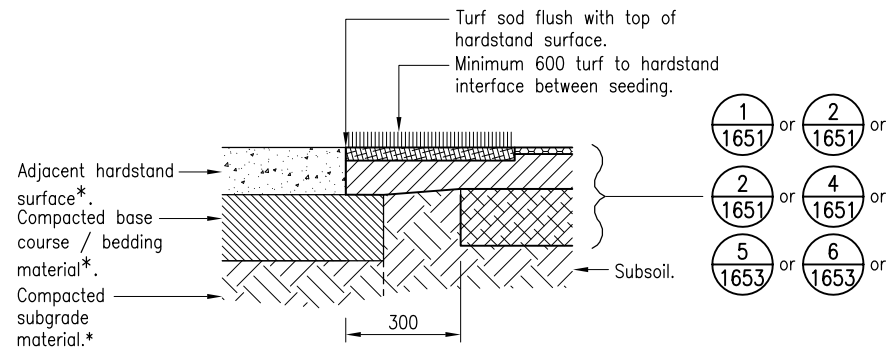
DETAIL 3 1644 HARDSTAND ABUTMENT TO SEEDING
