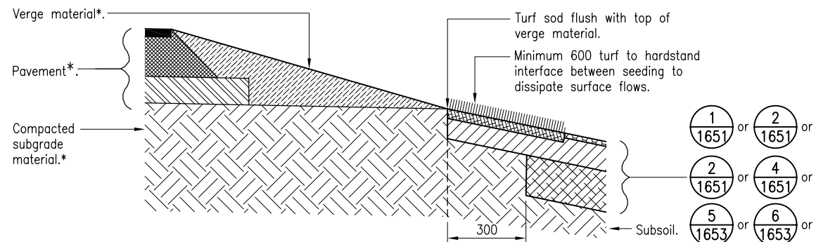
DETAIL 6 1644 VERGE TO SEEDING
