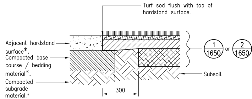
DETAIL 2 1644 HARDSTAND ABUTMENT TO TURF
