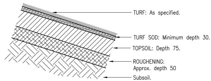
DETAIL 2 1650 TURF SLOPE > 1 ON 4
