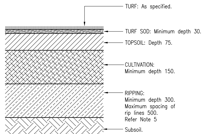
DETAIL 1 1650 TURF SLOPE \leq 1 ON 4
