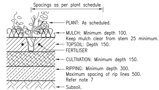
DETAIL 2 1653 PLANTING BROADACRE AREAS <25L CONTAINER SLOPE ≤ 1 ON 4
