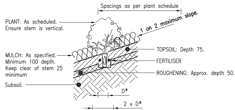
DETAIL 3 1653 PLANTING SLOPES TOPSOIL TO SLOPE <25L CONTAINER SLOPE > 1 ON 4
