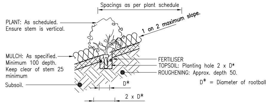
DETAIL 4 1653 PLANTING SLOPES TOPSOIL TO PLANTING HOLES <25L CONTAINER SLOPE > 1 ON 4
