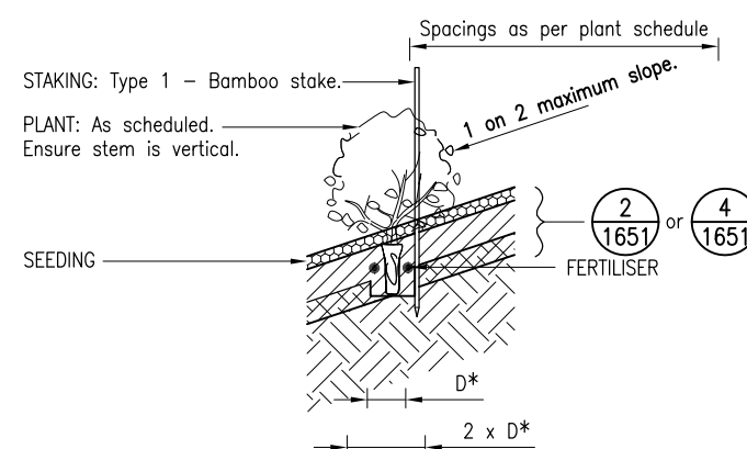
DETAIL 6 1653 SEEDING WITH PLANTING <25L CONTAINER SLOPE > 1 ON 4
