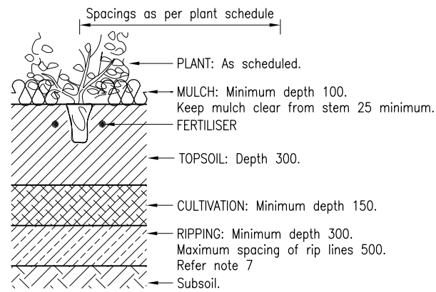
DETAIL 1 1653 PLANTING CONTAINED AREAS <25L CONTAINER SLOPE ≤ 1 ON 4
