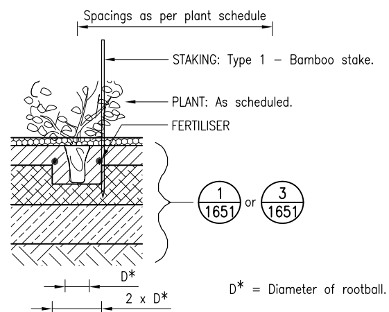
DETAIL 5 1653 SEEDING AREAS WITH PLANTING <25L CONTAINER SLOPE ≤ 1 ON 4
