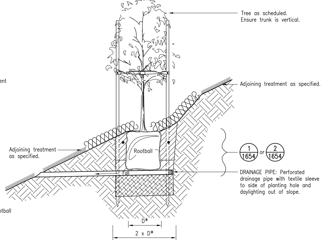
DETAIL 4 1654 PLANTING SLOPES ≥25L CONTAINER SLOPE > 1 ON 4 POOR DRAINING SOILS
