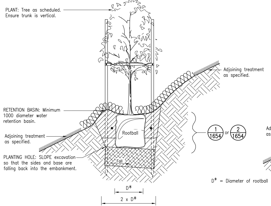
DETAIL 3 1654 PLANTING SLOPES ≥25L CONTAINER SLOPE > 1 ON 4 FREE DRAINING SOILS
