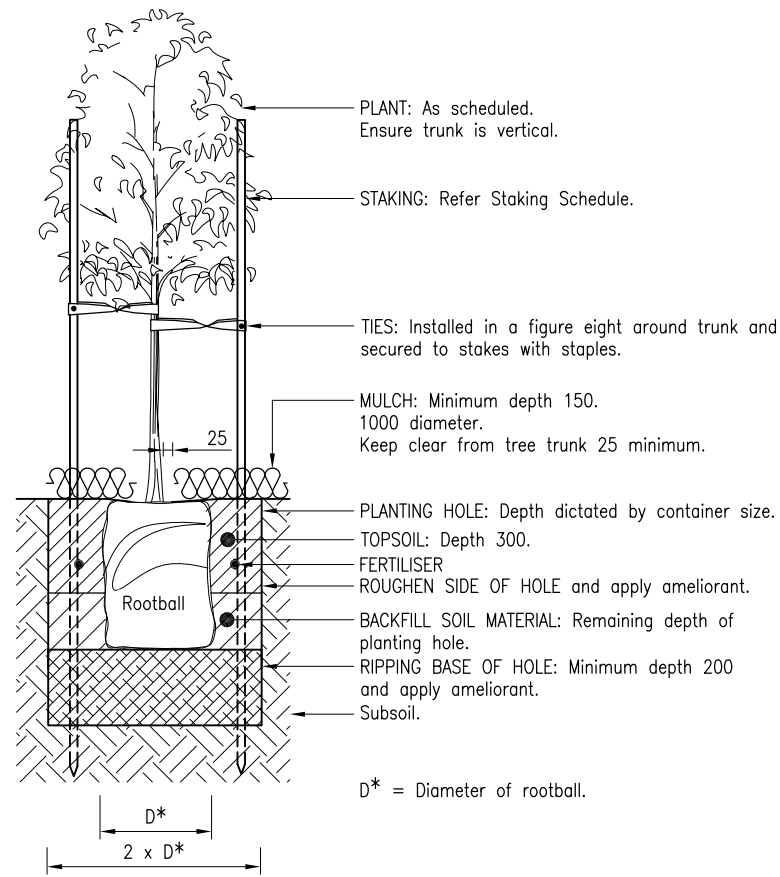
DETAIL 1 1654 PLANTING MULCHED AREAS ≥25L CONTAINER SLOPE ≤ 1 ON 4
