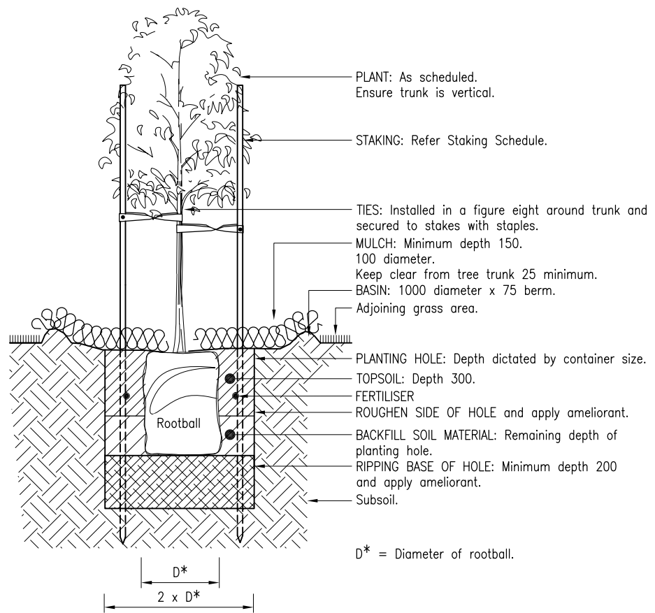
DETAIL 2 1654 PLANTING GRASS AREAS ≥25L CONTAINER SLOPE ≤ 1 ON 4
