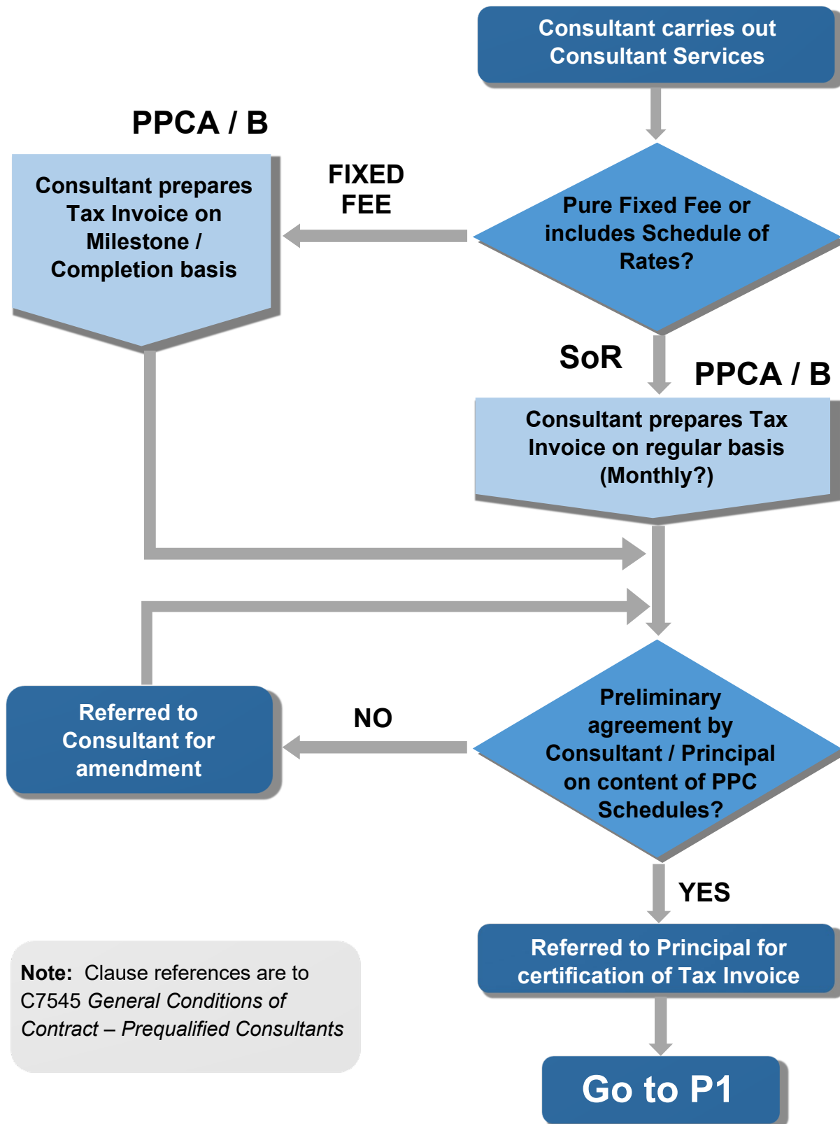
Figure 3.4 – Payment flowchart
