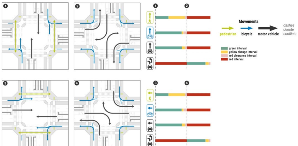
Figure 4.5.2(d) – Protected bicycle phase
