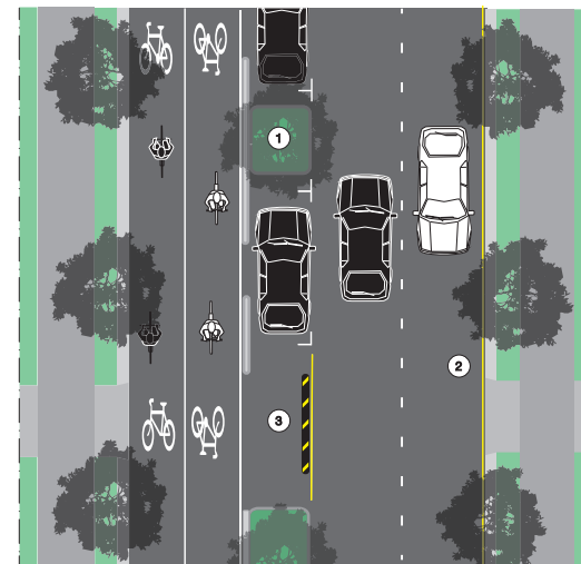
One x 2 way separated cycle track (preferred)
