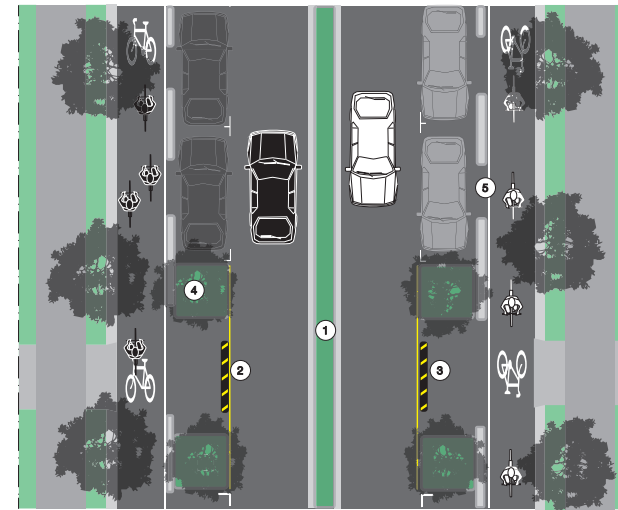
Two x 1-way separated cycle track (narrow with car parking)
