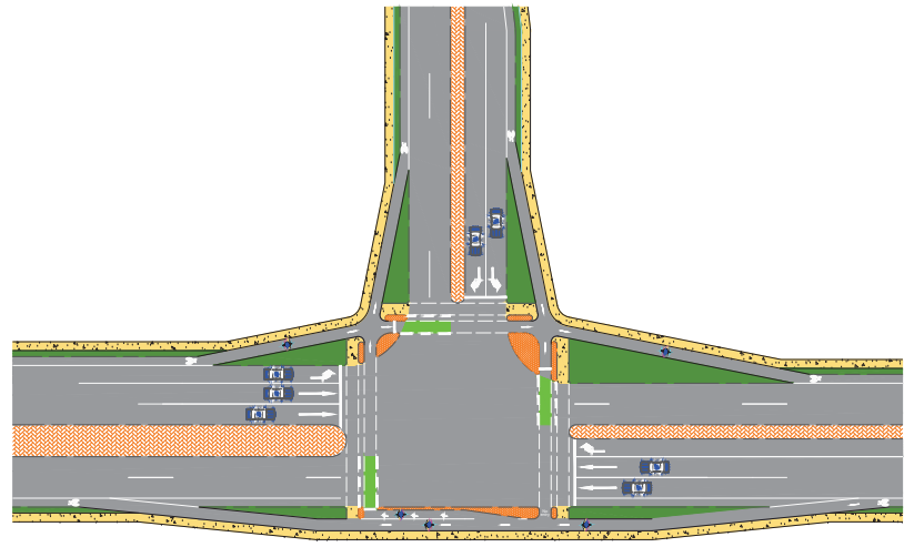
Bicycle lane transition to cycle track
