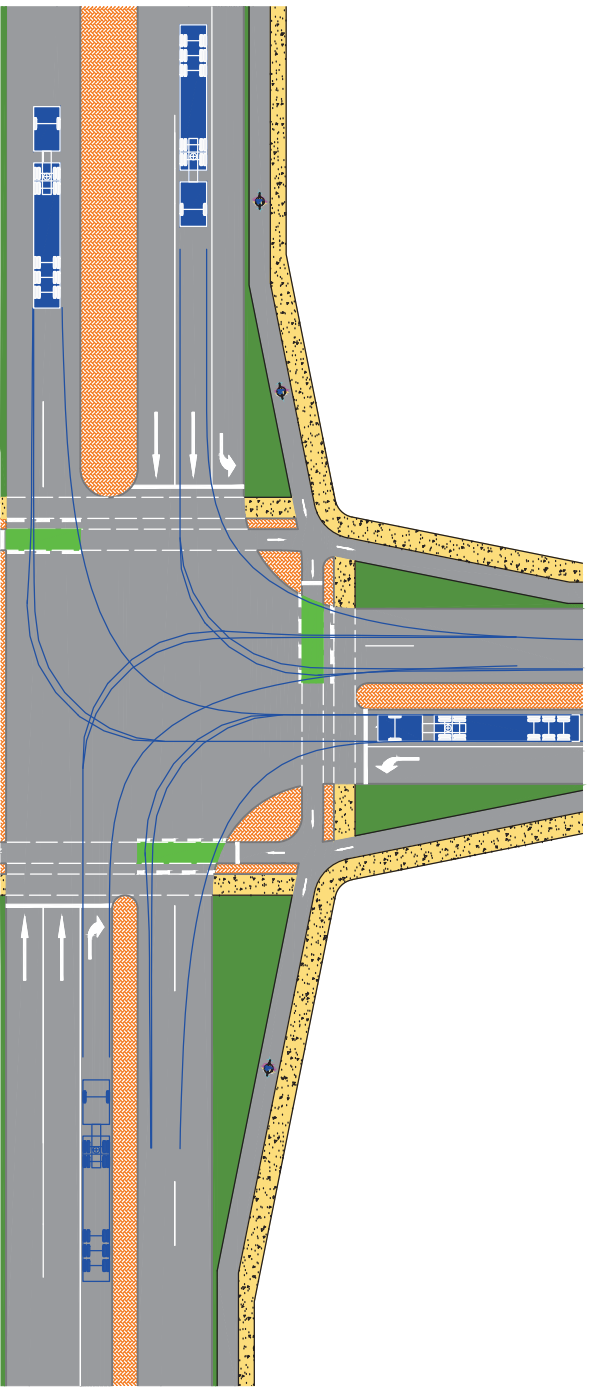
Turning movements: Service vehicle (R12.5m)
