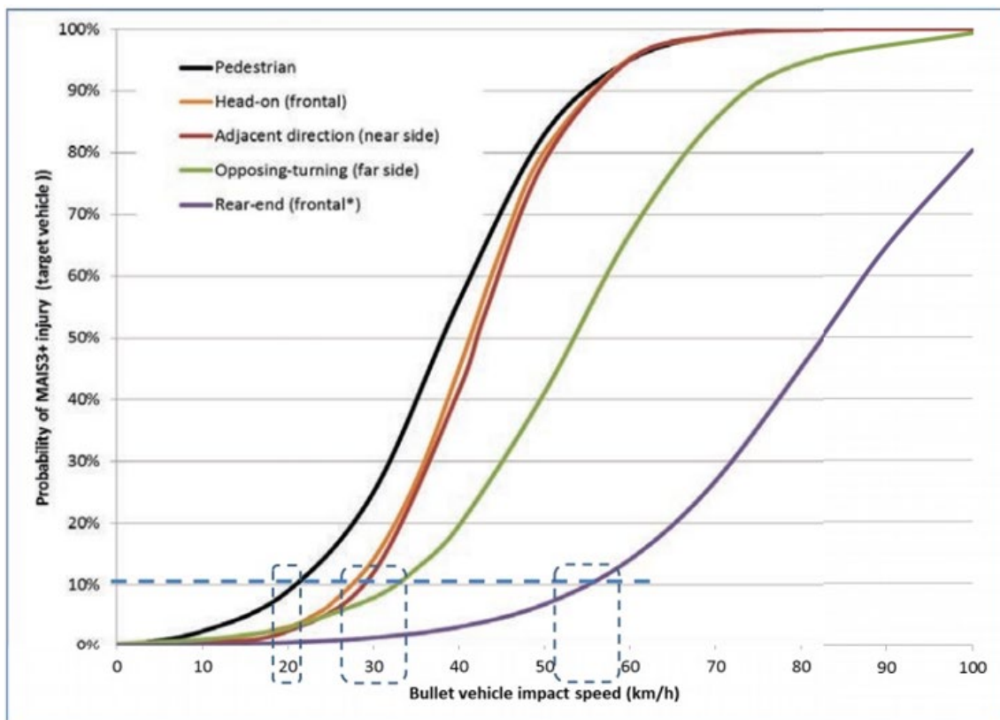
Figure 1.2(c) – Probability of fatal or serious injury vs. vehicle impact speed
