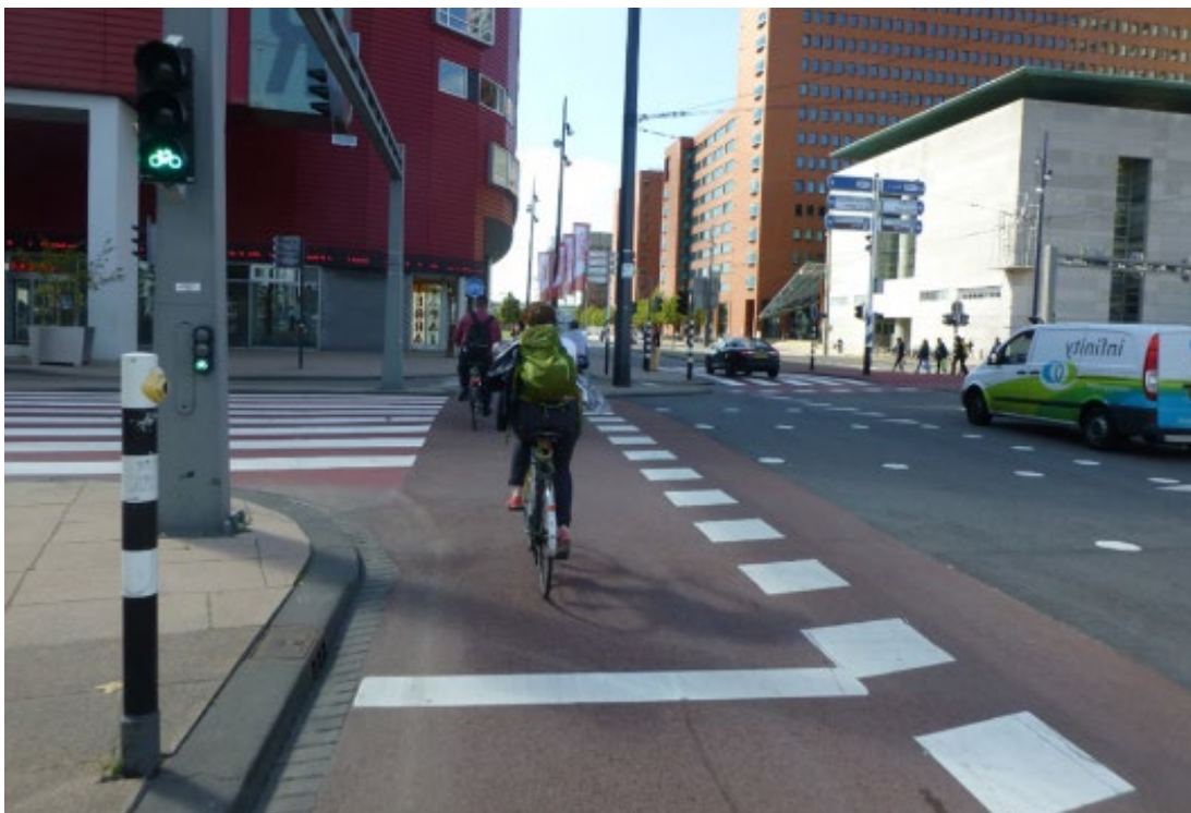
Figure 4.5.2(g) – Push button conveniently located 200 mm from cycle track at signalised intersection with advanced stop line, Rotterdam
