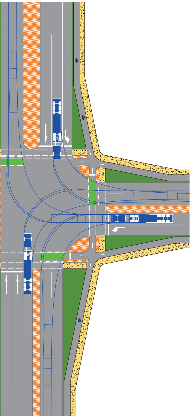
Turning movements: 19m semi (R12.5m)
