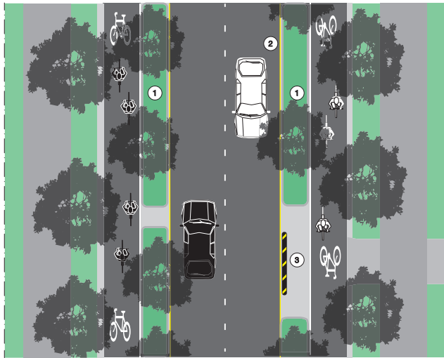
Two x 1-way separated cycle track (preferred)
