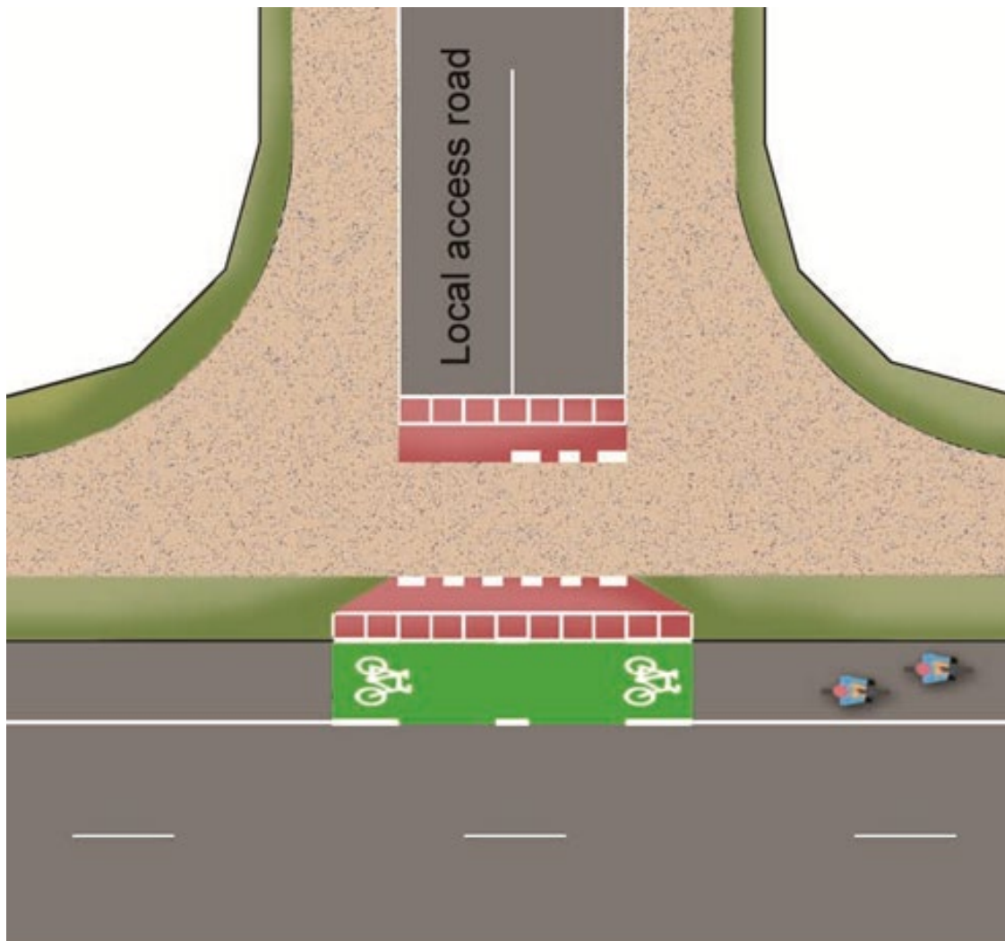
Figure 4.3.1(c) – Bicycle lane and at-grade footpath at side road (LTS2)
