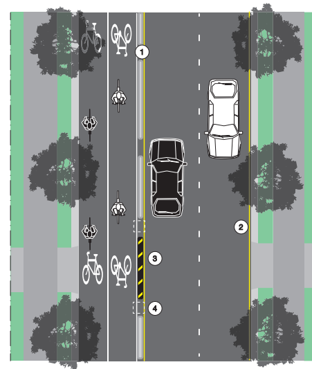
Two x 2-way separated cycle track (preferred)
