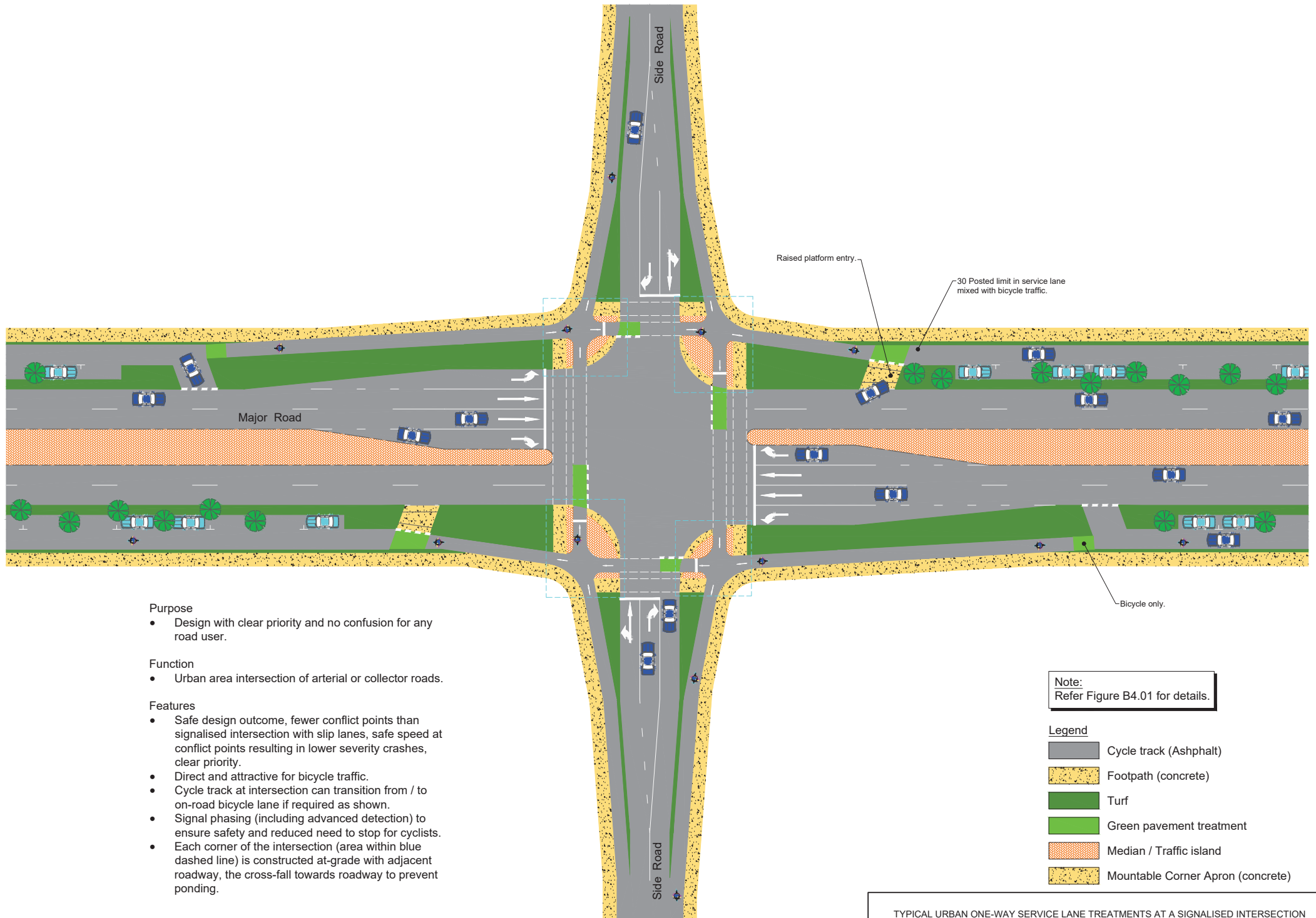
TYPICAL URBAN ONE-WAY SERVICE LANE TREATMENTS AT A SIGNALISED INTERSECTION
