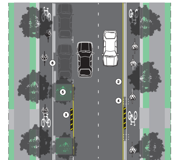
Two x 1-way separated cycle track (narrow with car parking) LTS1
