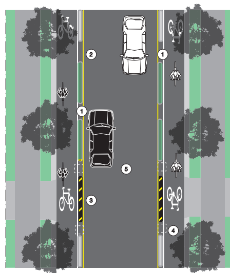
Two x 1-way separated cycle track (preferred)
