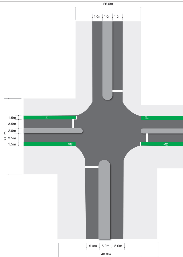
EXISTING SIGNALISED INTERSECTION LTS4
