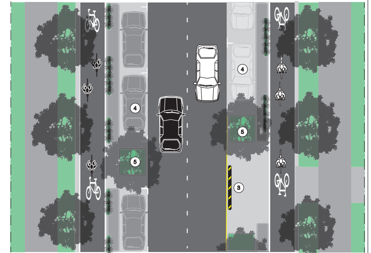
Two x 1-way separated cycle track with parking both sides (preferred)
