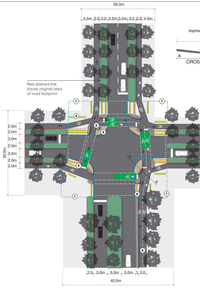
RETROFIT SIGNALISED INTERSECTION LTS1
