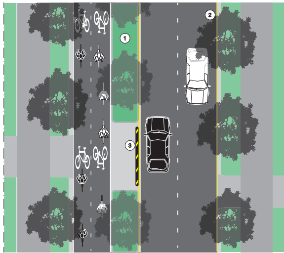
One x 2-way separated cycle track (preferred)
