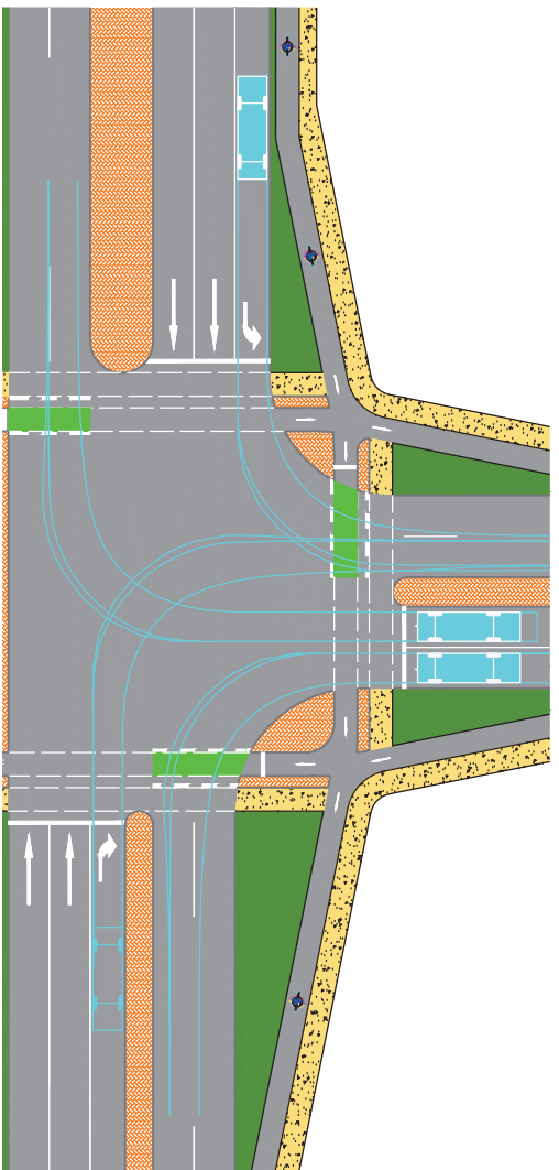
Turning movements: Service vehicle (R12.5m)
