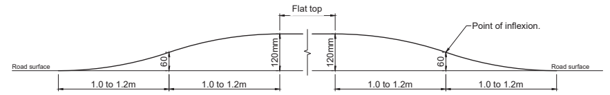
Section B-B: Sinusoidal raised platform profile
