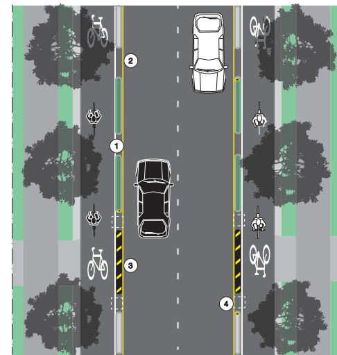
Two x 1-way separated cycle track (preferred)
