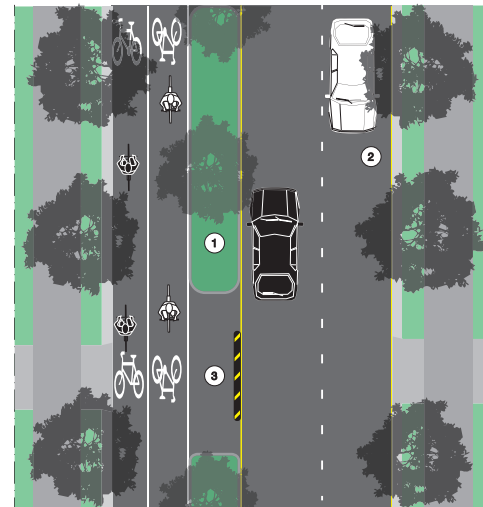
One x two-way separated cycle track (preferred)
