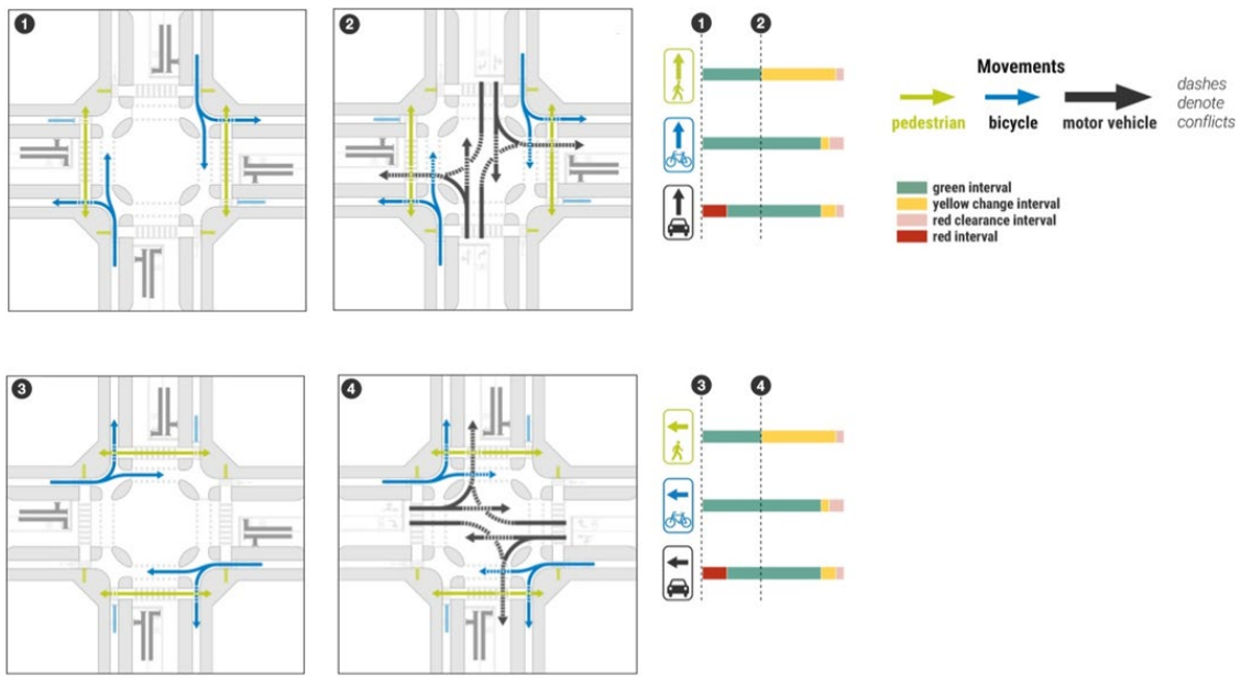
Figure 4.5.2(d) – Protected bicycle phase
