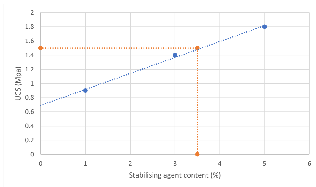
Figure 8.4.8 – Stabilising agent content v UCS at 28 days
