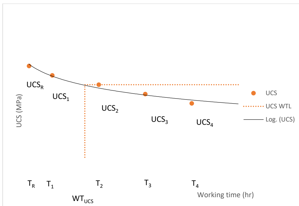
Figure 2 – Working time for UCS
