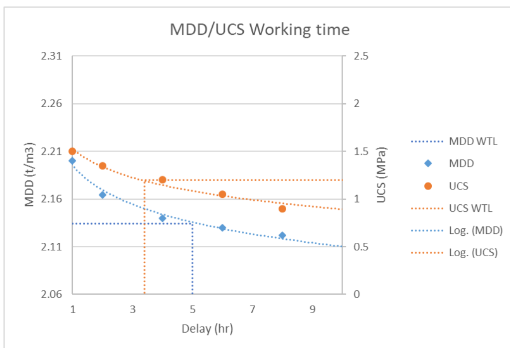
Figure 3.4.9 – MDD / UCS v delay
