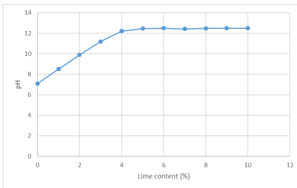
Figure 7.4.3 – Lime demand curve
