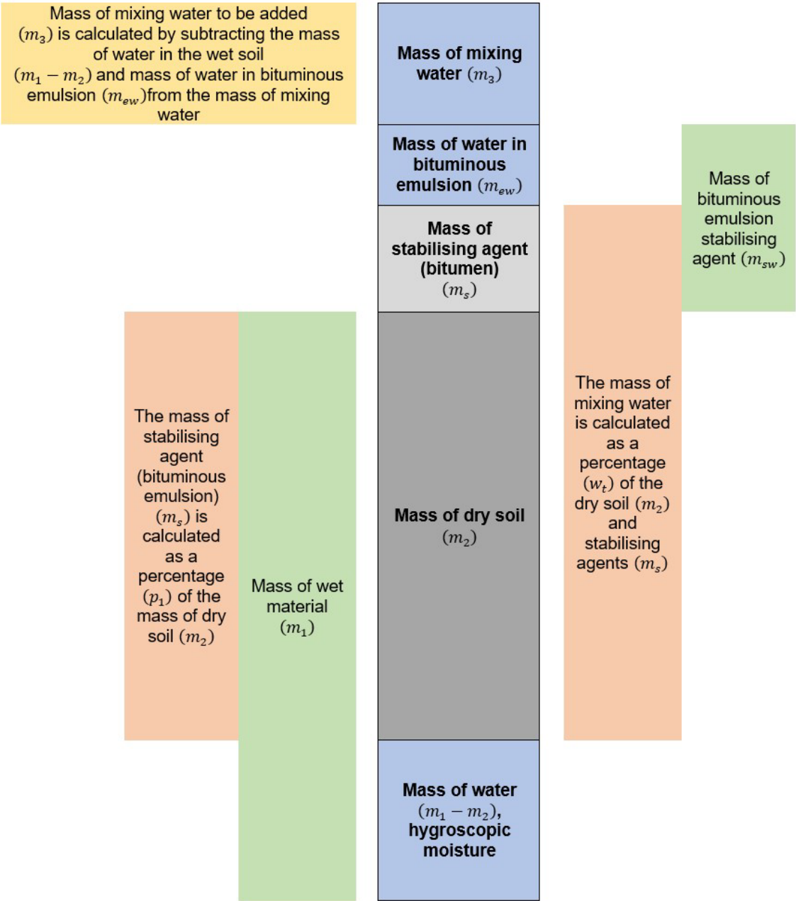
Figure 2 – Example of mass relationships for bituminous emulsion
