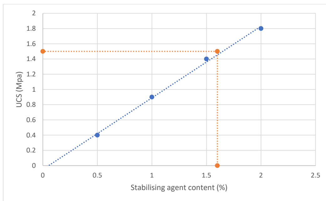
Figure 3.4.8 – Stabilising agent content v UCS
