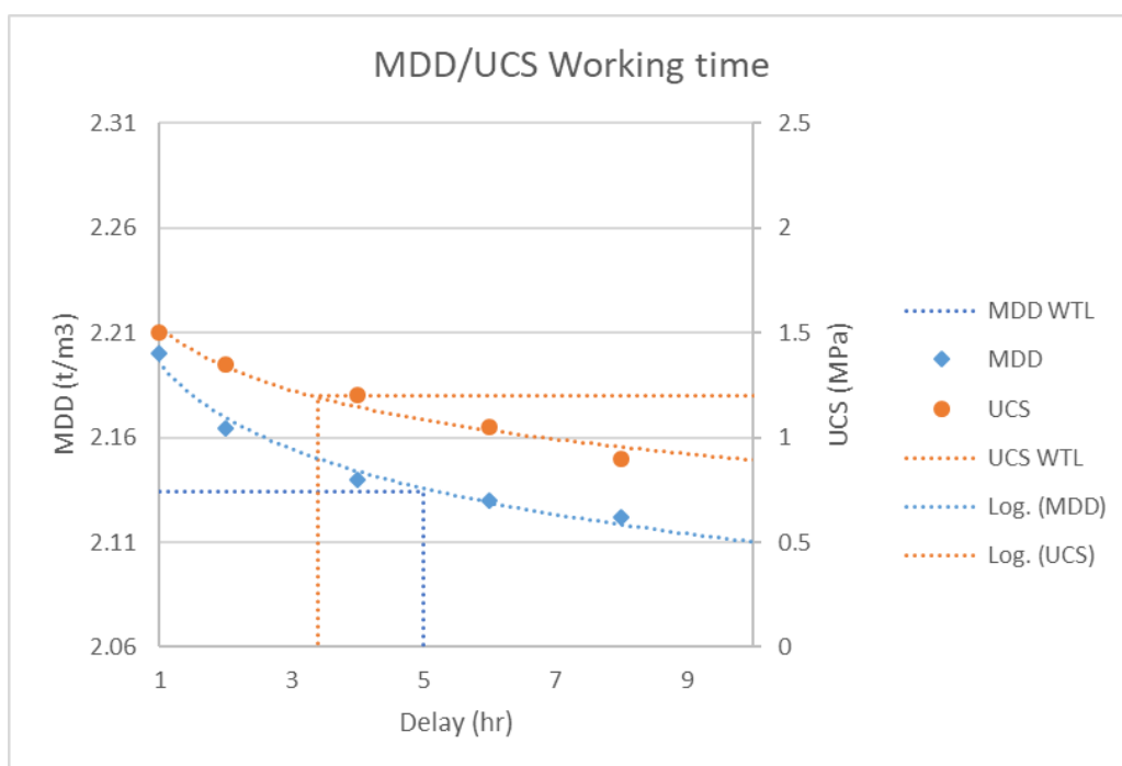
Figure 8.4.9 – MDD / UCS v delay
