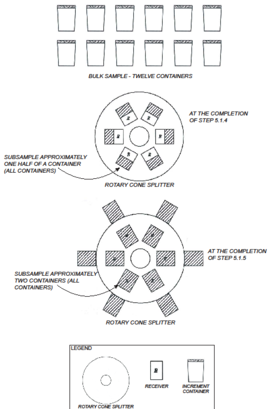
Figure 2 – Total sample combination by rotary cone
