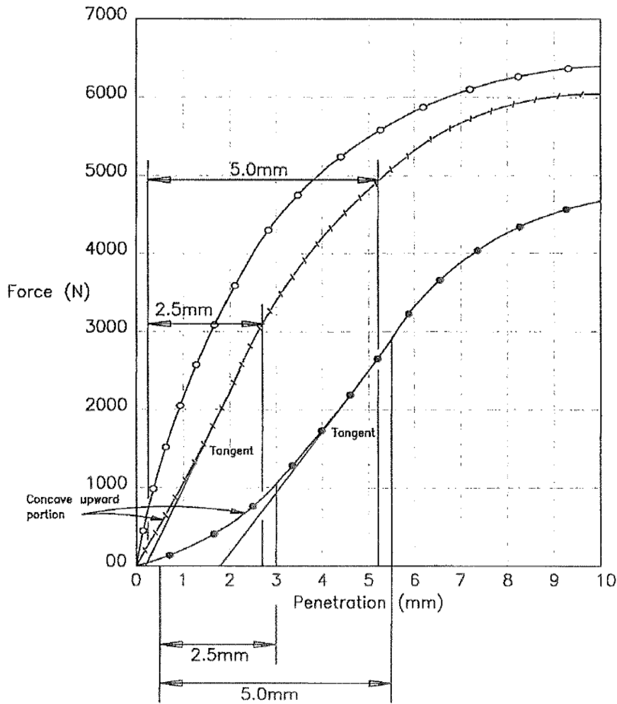
Figure 1 – Typical force – penetration curves showing the determination of new penetration
