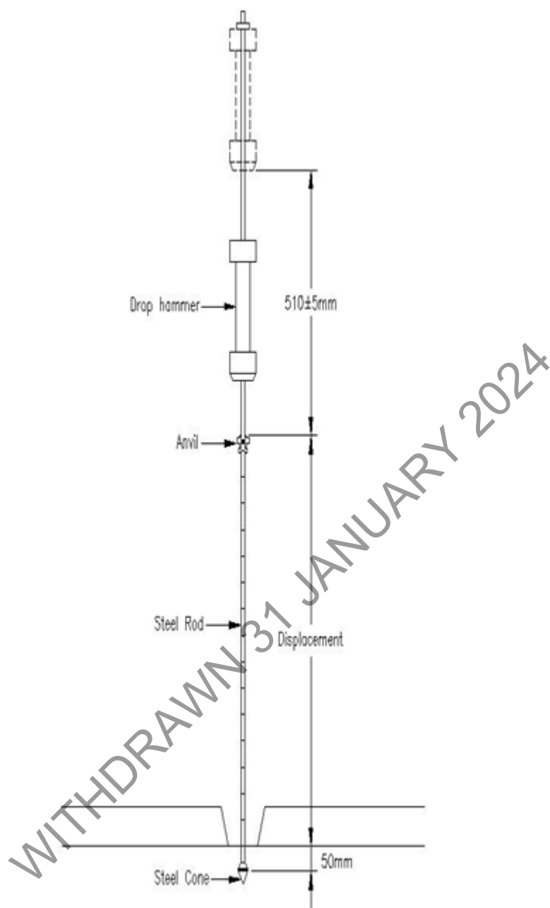
Figure 1 – Initial embedment of dynamic cone penetrometer
