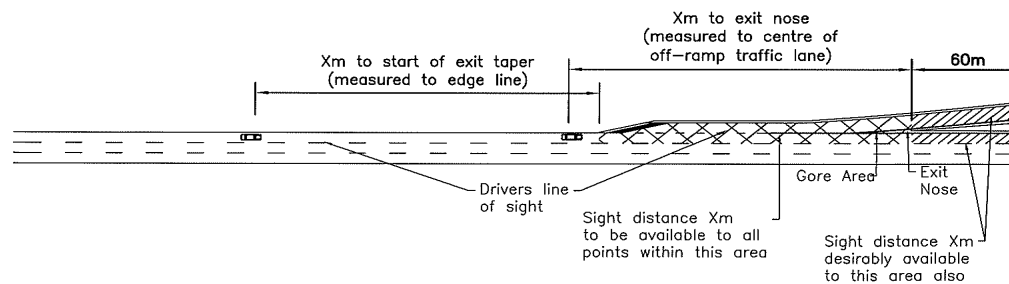
(b) Plan – exit taper
