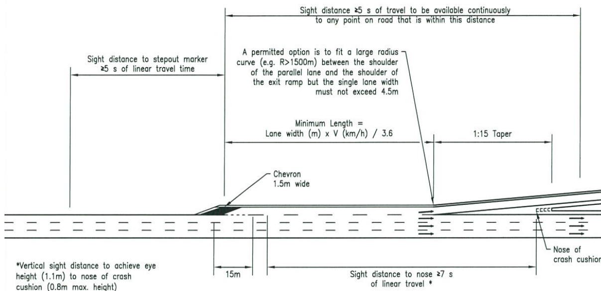
Figure 11.2(d) – Example of exit from an arterial road
