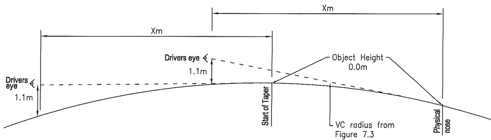
Figure 7.2 – Sight distance requirements at exit ramps
