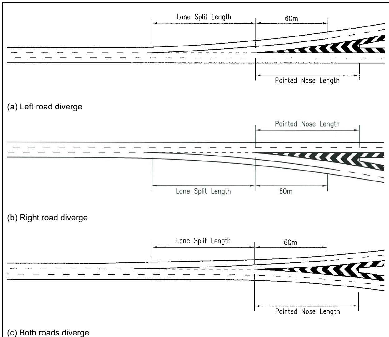
Figure 11.2(c) – Example of 2-lane exit for a freeway or major divided road
