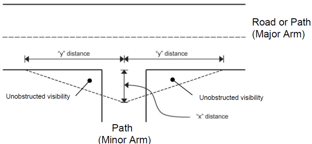
Figure 6A-2 – Visibility splays at intersections with paths
