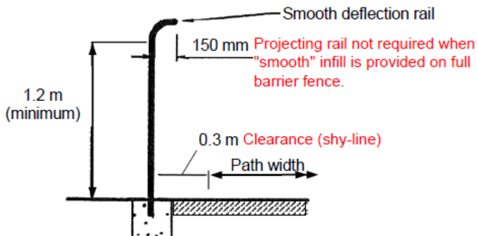
Figure 6A-1 - Example of full barrier fence (Section A-A)
