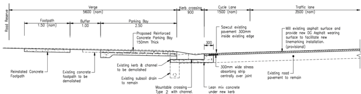
Figure 6B-18 – Example cross-section and layout for verge car parking
