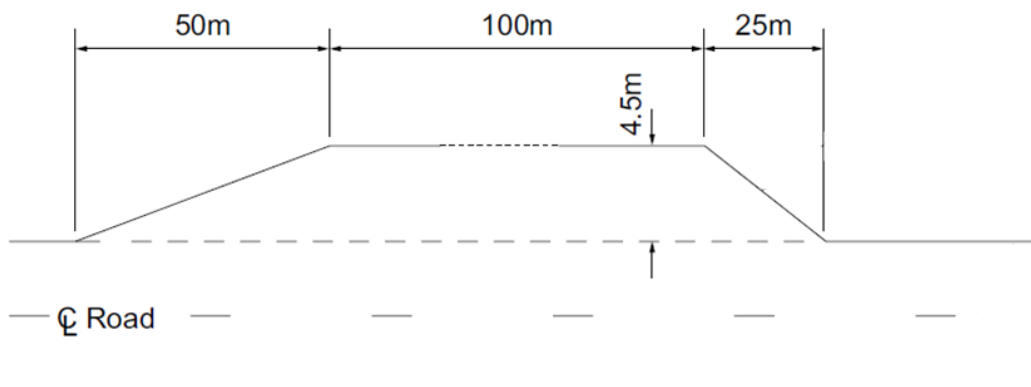
Figure 6B-7 – Heavy vehicle stopping place typical dimensions
