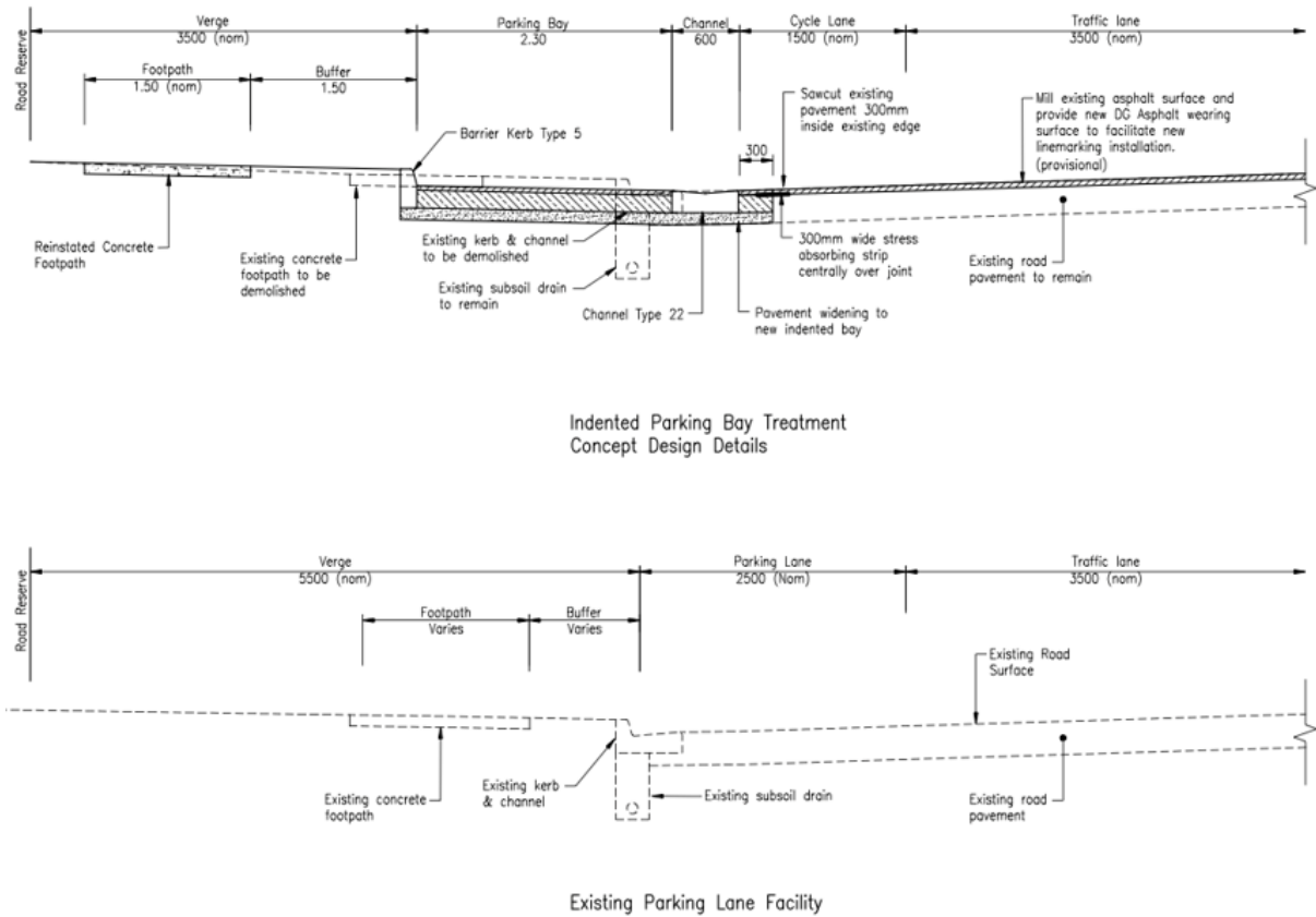
Figure 6B-19 – Example cross-section for indented car parking
