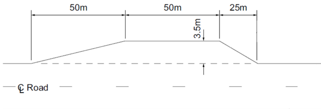
Figure 6B-6 – Passenger vehicle stopping place typical dimensions
