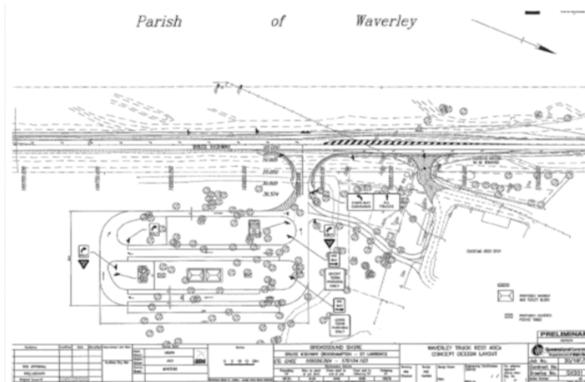
Figure 6B-15 – Dual-use rest area design
