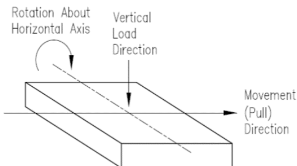
Figure 6.5.4 – Definition of loads directions in bearing elevation
