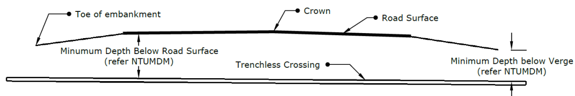
Figure 5.2.2(a) – Minimum depth below single carriageway
