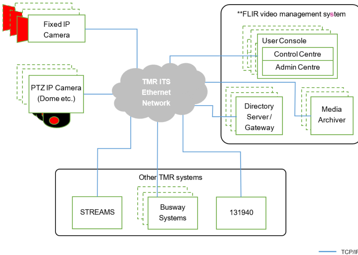
Figure 7.1 – High Level Video System Architecture
