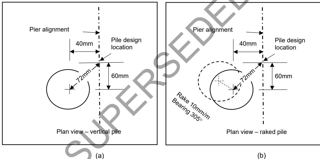
Figure 12.7.1 - Example of As Constructed Survey and conformance results of piles
