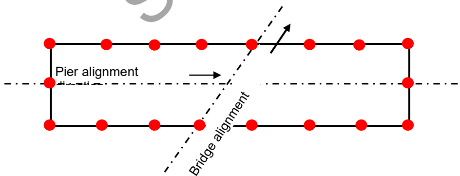
Figure 12.7.2.3 - Example of linearity or planarity As Constructed Survey and conformance locations for headstock
