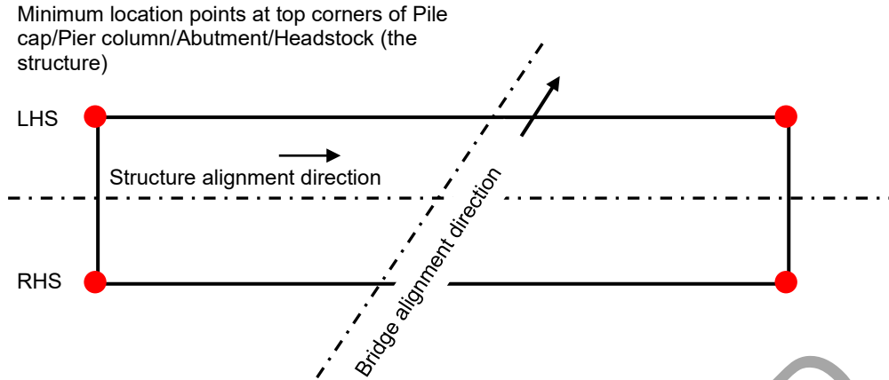
Figure 12.7.2.1 - Example of As Constructed Survey and conformance locations of pile caps / pier columns / abutments and headstocks
