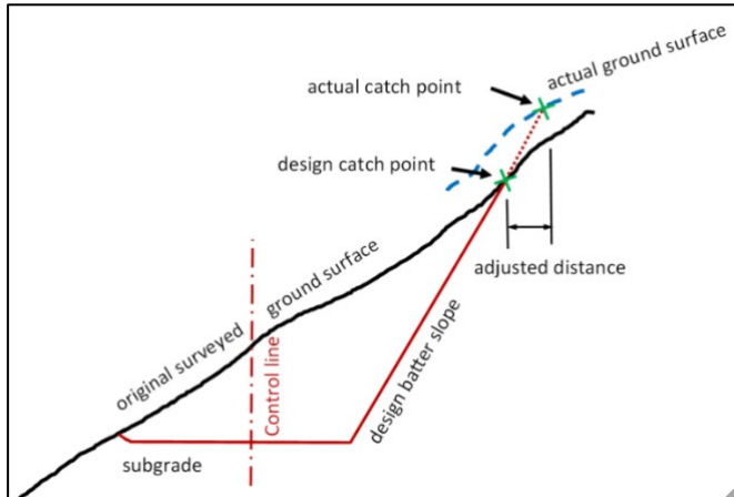
Figure 9.3.2 – Excavation catch point
