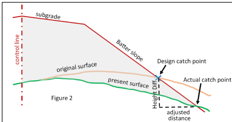
Figure 9.3.3 – Embankment catch point
