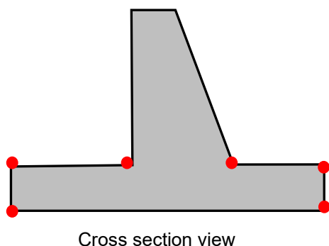
Figure 12.4.1 - Typical cross section of As Constructed Survey and conformance locations of concrete retaining wall
