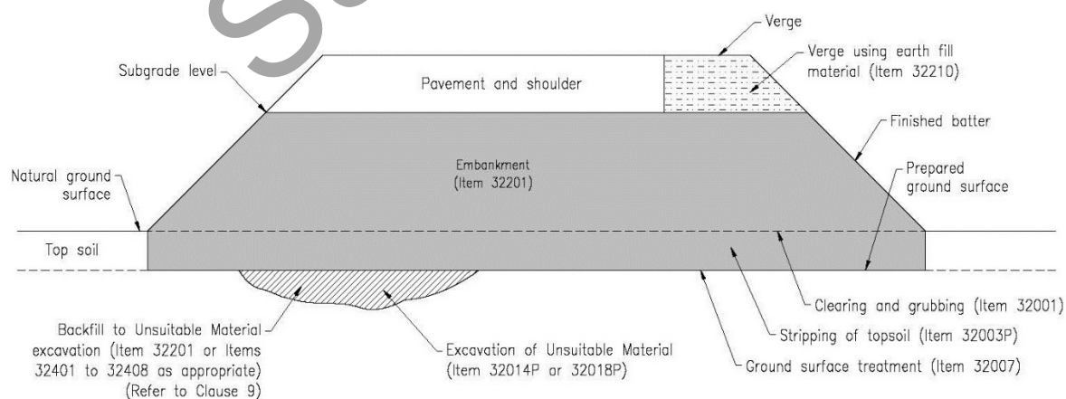
Figure 2.1(b) – Embankment
