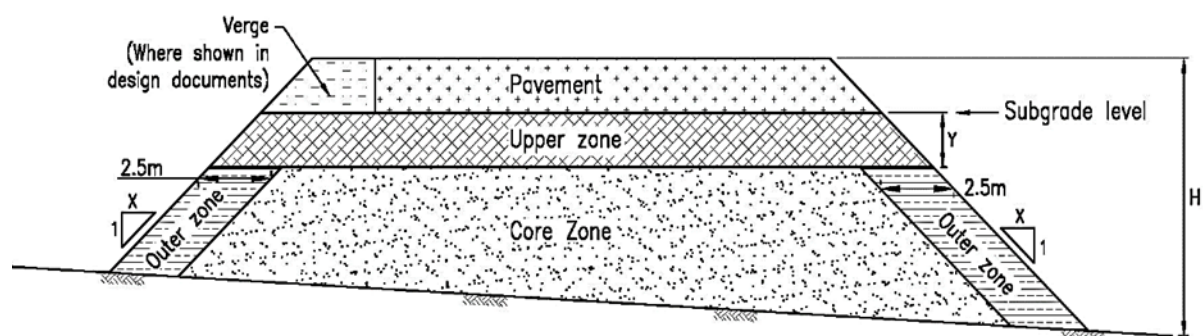
Figure 14.3.1 – Embankment zones
