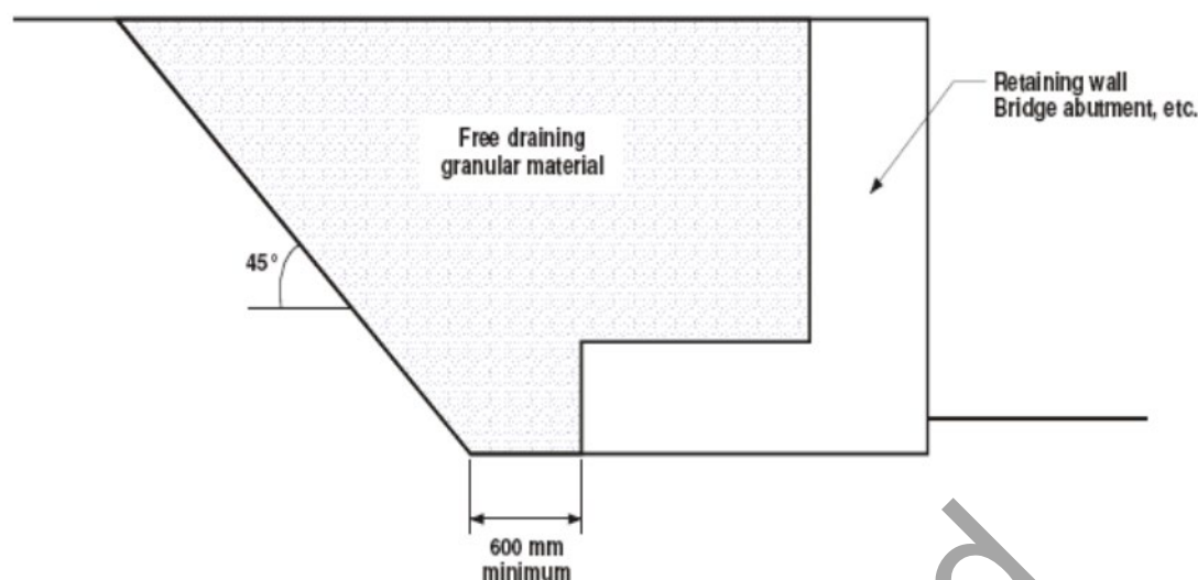
Figure 19.3.5 – Minimum extent of Free-Draining Granular Material behind soil retaining structure
