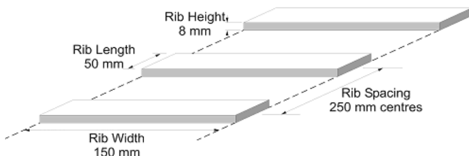
Figure 7.7.3(a) – ATLM edge line
