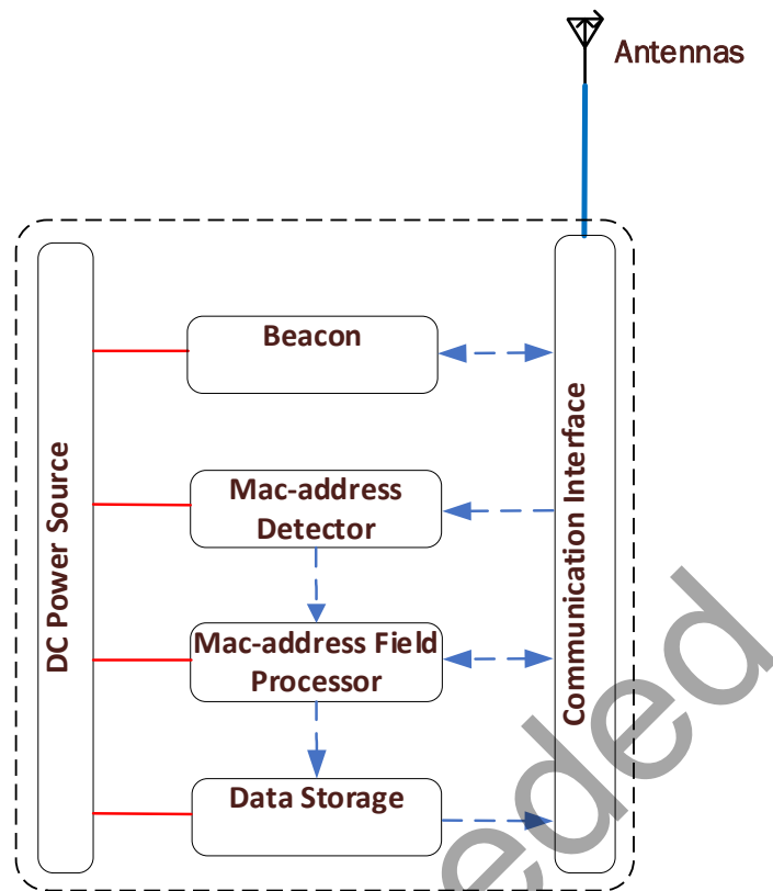
Figure 5.1 – WTS components
