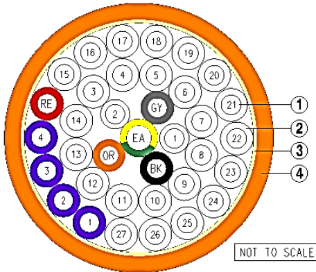
Figure 6.5 – 36-core cable
