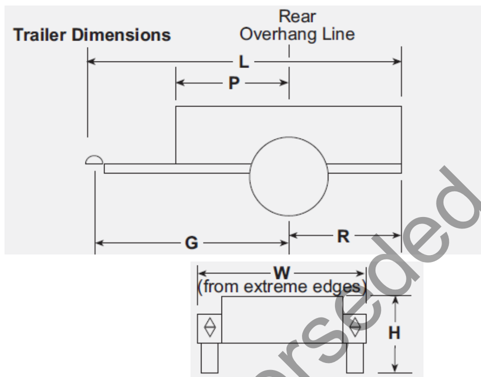
Figure 10.2.3 – Trailer dimensions
