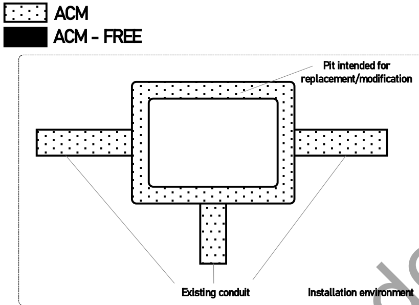
Figure 6.1.1(c) – Scenario 3: ACM pits and conduits
