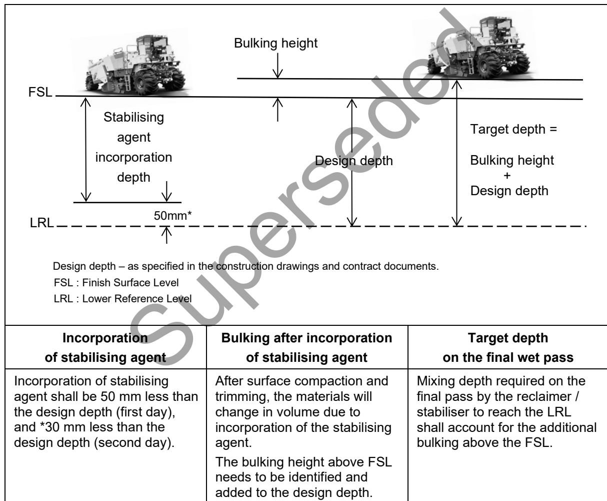
Figure 8.7.6.4 – Target depth sketch
