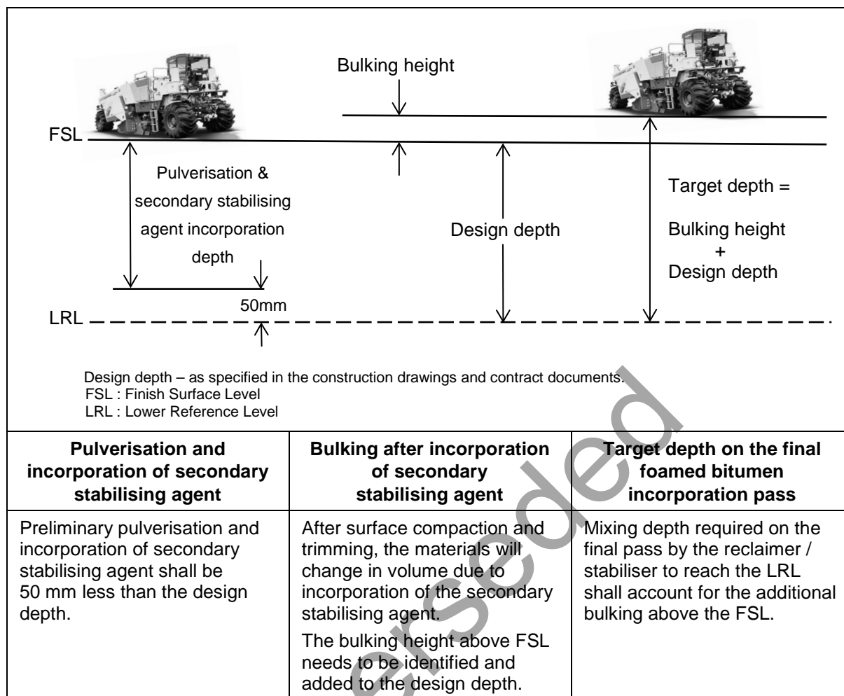
Figure 8.7.11 – Target depth sketch
