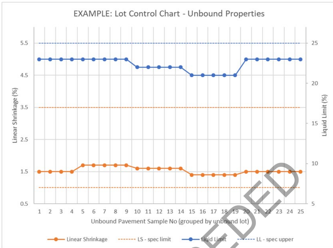
Figure B2 – Example: Lot Control Chart – Unbound Properties
