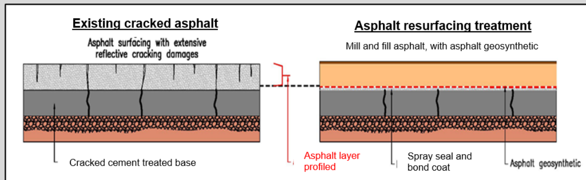
Figure 1(e) – Typical asphalt inlay (or 'mill and fill') reflective cracking treatment
