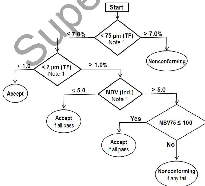
Figure 6.1 - Fine aggregate requirements
