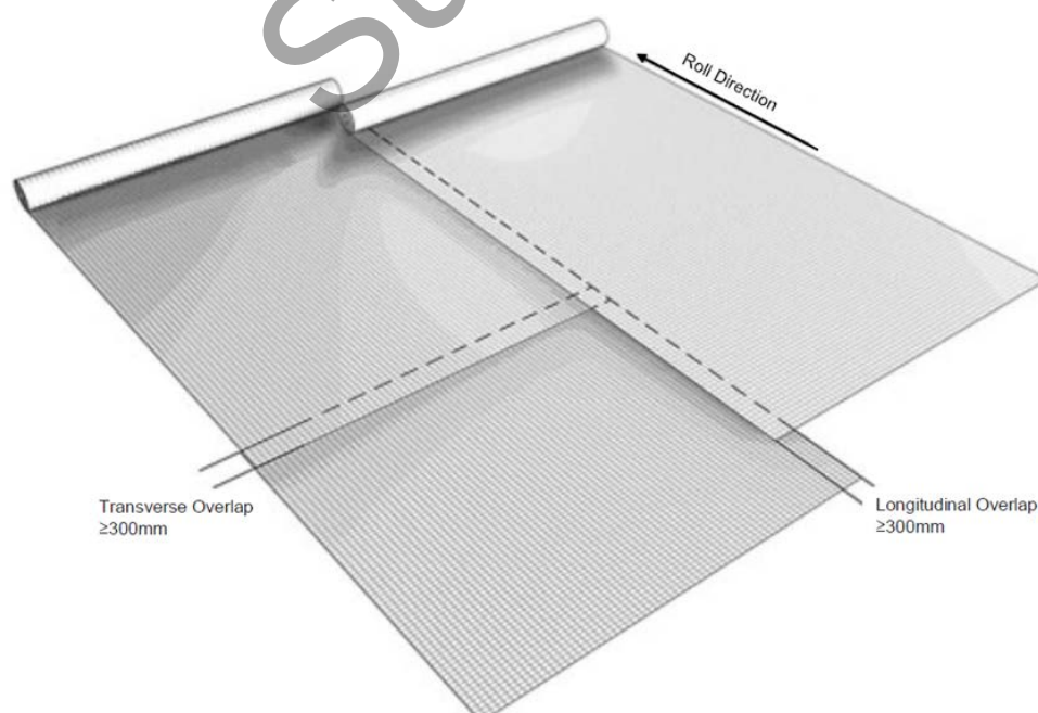
Figure 8.1(a) – Minimum overlap
