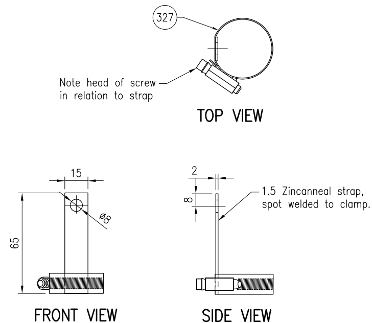
DETAIL 1 CABLE CLAMP SUPPORT
