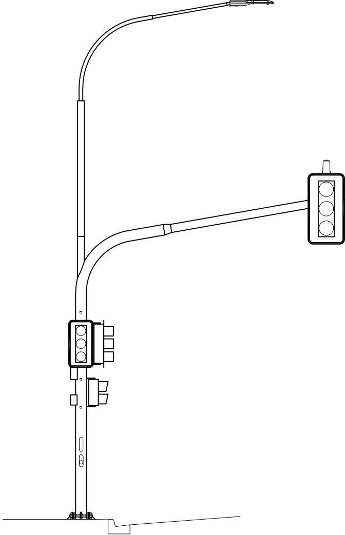
COMBINATION TRAFFIC SIGNAL MAST ARM AND ROAD LIGHTING POLE Refer Standard Drawing 1427
