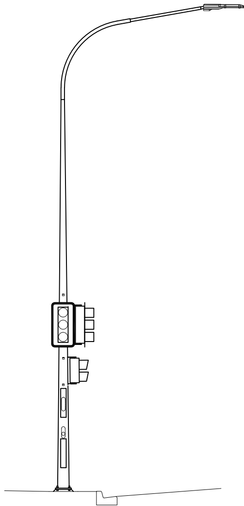
JOINT USE TRAFFIC SIGNAL AND ROAD LIGHTING POLE Refer Standard Drawing 1377
