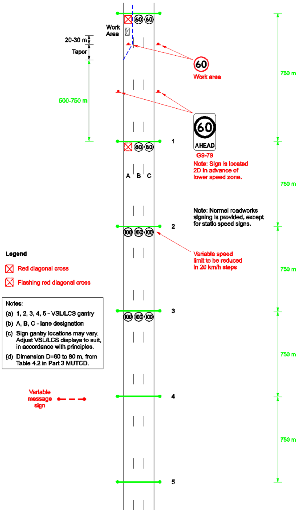
Figure 2.6(d) – Work in one lane – 500–750 m
