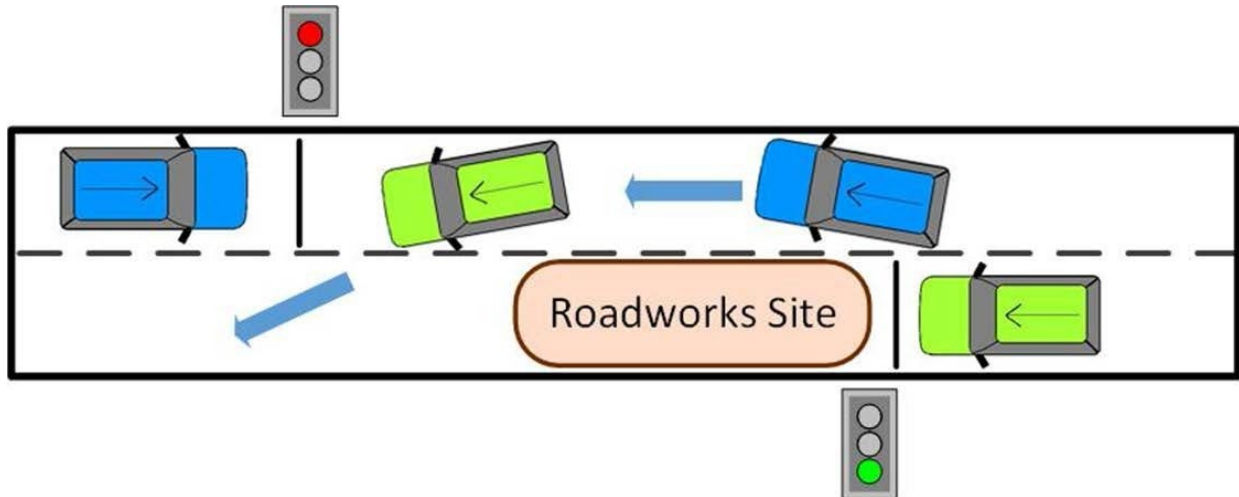
Figure 2.5.5.1 – Shuttle control
