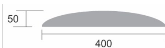
Figure 1.6.7 – Speed hump profile
