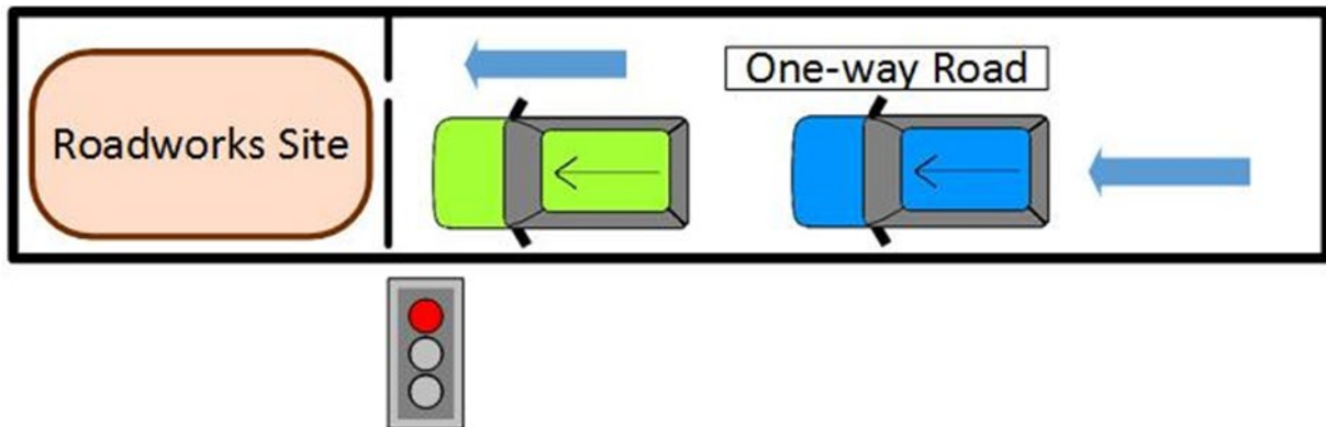
Figure 2.5.5.3 – Gating control
