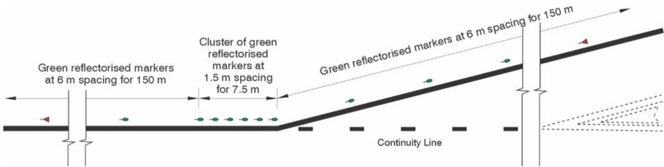
Figure 5.11.7 – Marking at an exit ramp
