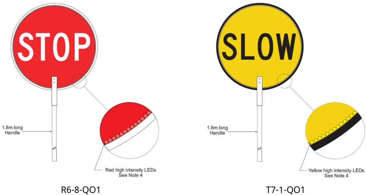
Figure 4.7.2 – LED-enhanced STOP / SLOW bat
