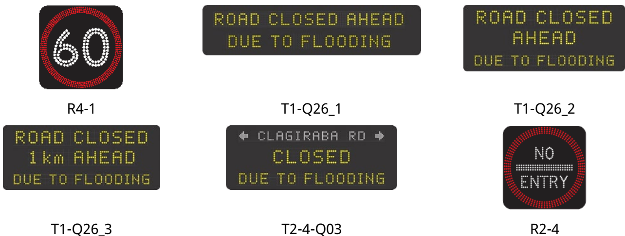
Figure 4.24 - Examples of electronic signs
