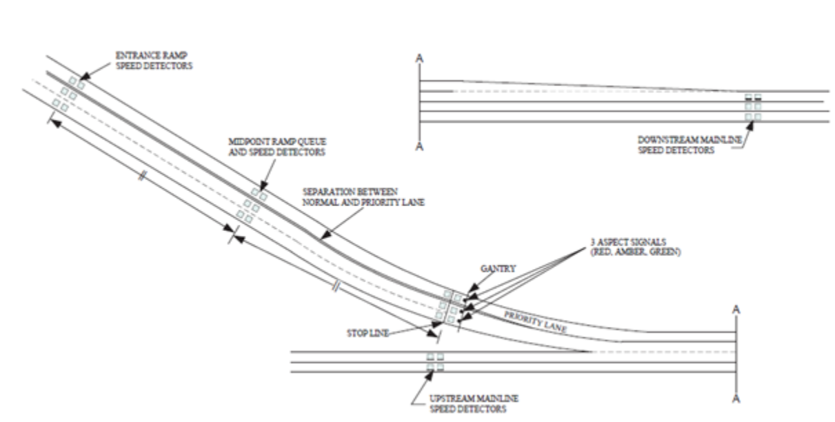
Figure 6.1.2.2(d) – Complex entry-ramp, 2 lanes of metered traffic and a metered priority lane
