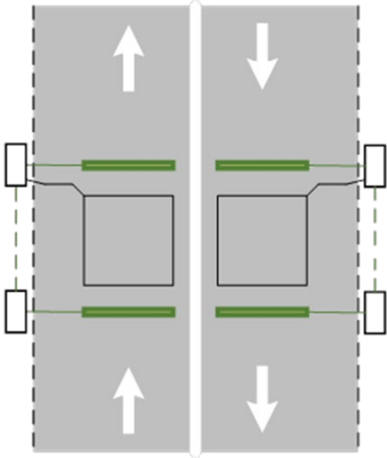
Figure 8.3.1 – Single lane bi-directional carriageway (Piezo-Loop-Piezo configuration for weigh-in-motion sites)
