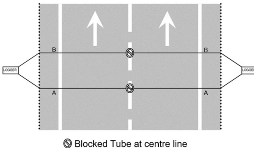
Figure 7.3.1.2 – single carriageway uni-directional site
