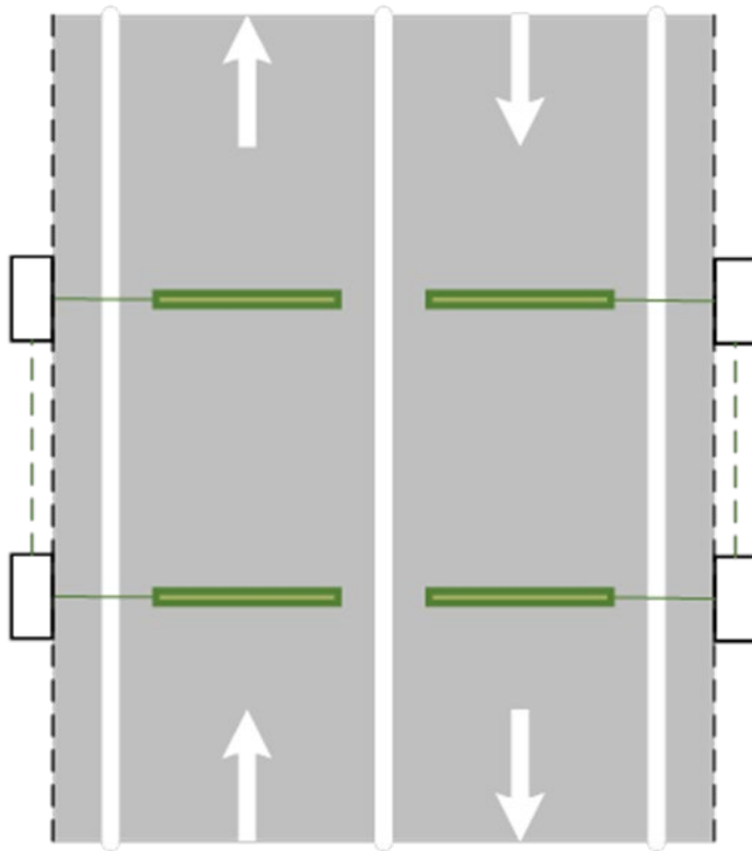
Figure 7.3.2.2.3 – Typical piezo-piezo configuration on single carriageway bi-directional road
