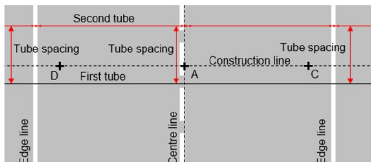
Figure 7.4.2(b) – Pneumatic tube installation details (determining the location of tubes)
