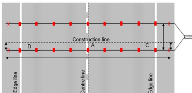
Figure 7.4.2(f) – Pneumatic tube installation details (tube final securing)
