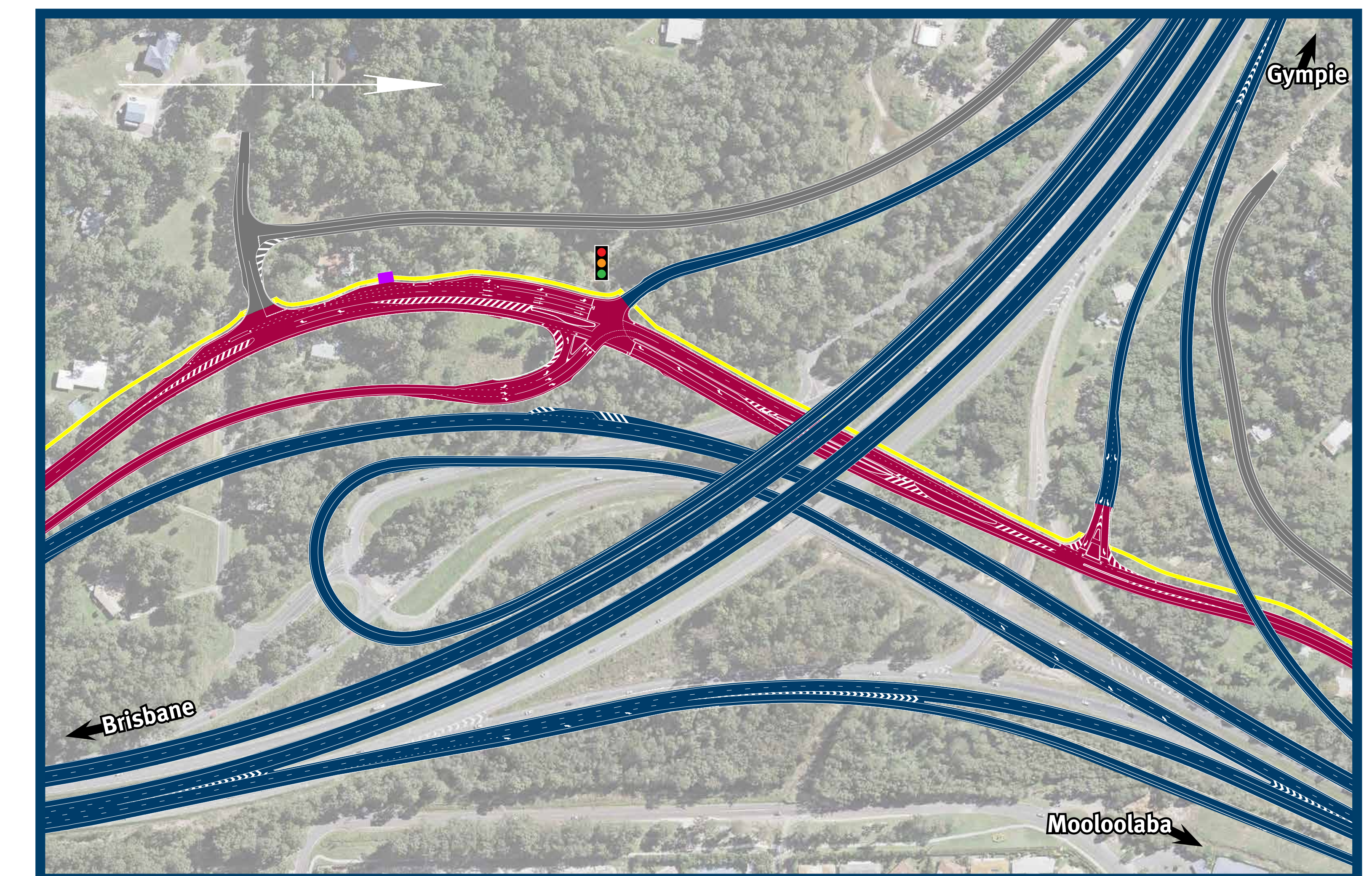
Inset C Sunshine Motorway interchange
