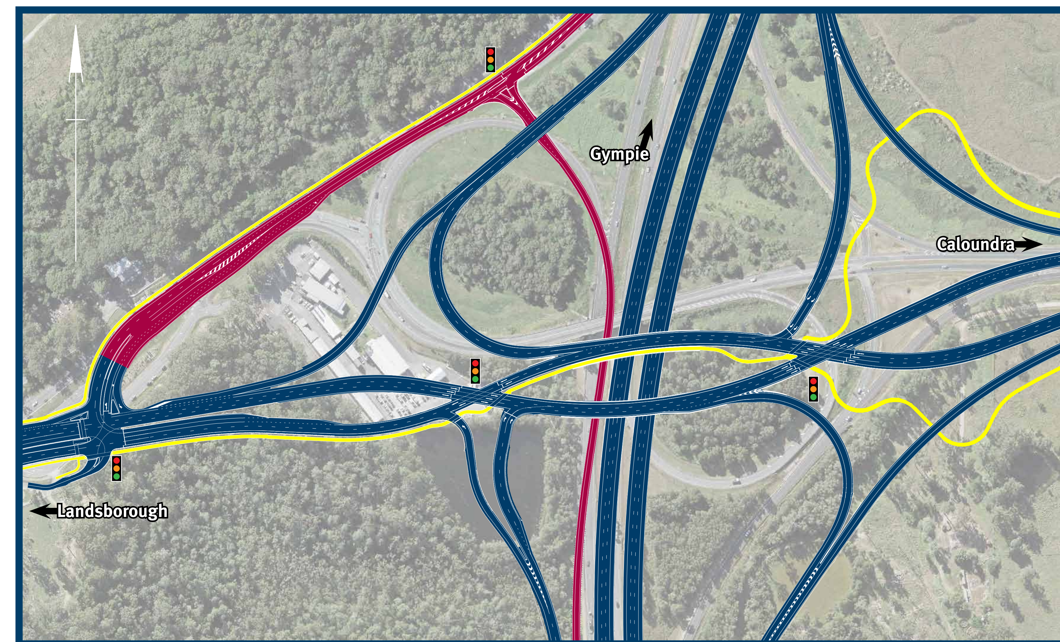
Inset A Caloundra Road interchange
