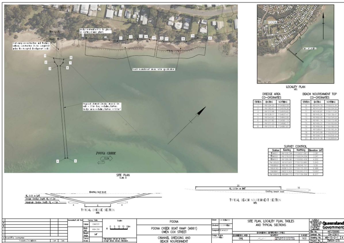
Proposed access channel location and beach nourishment areas
